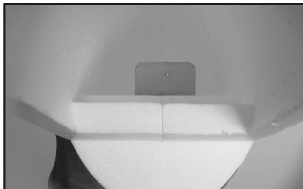
4. Next fit the pushrod support in fuselage. Note the orientation of the hole as it is not in the center.
