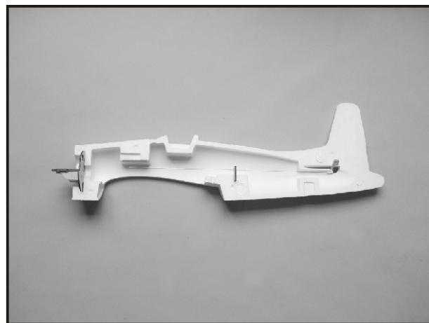
5. Insert pushrod through the push rod support then thread the small clevis then snap on the elevator joiner. Epoxy the fire wall assembly and pushrod support in place of right fuselage.
