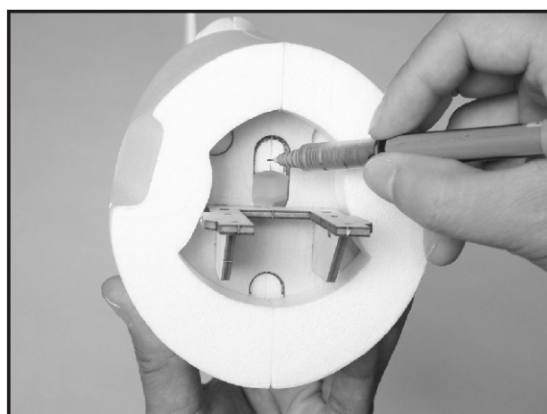
3. You may need to remove the foam flashing from fuselage and wing. Trial fit the firewall assembly in fuselage. Mark guide lines on fuselage which will help you to position the firewall assembly in place correctly later.
