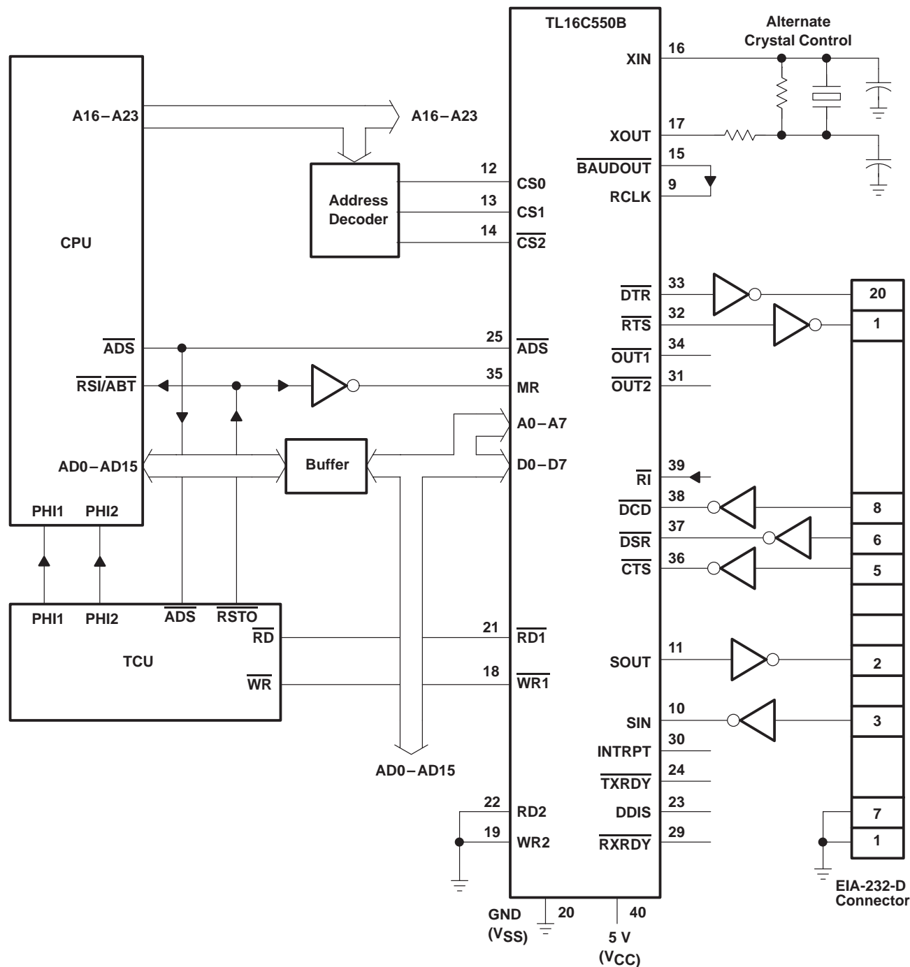
Figure 15. Typical TL16C550B Connection to a CPU
