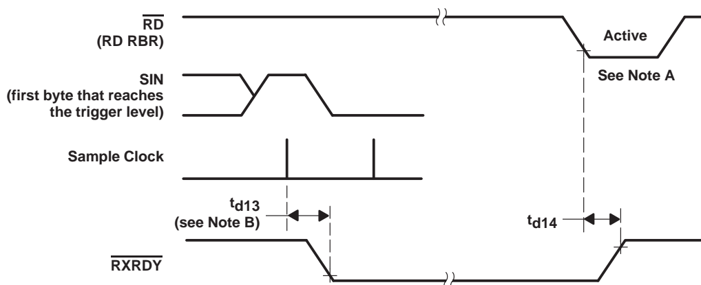
Figure 7. Receiver Ready ( \overline{\text{RXRDY}} ) Waveforms, \text{FCR0} = 0 or \text{FCR0} = 1 and \text{FCR3} = 0 (mode 0)
