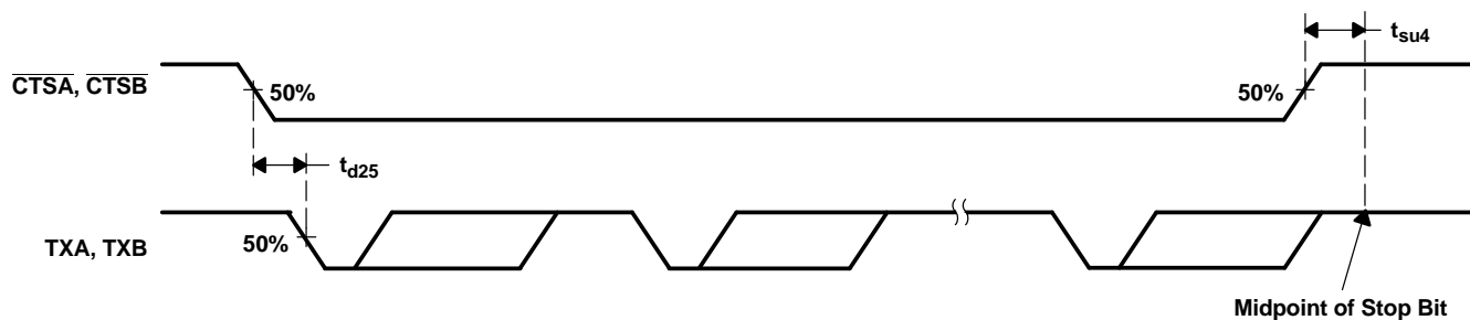
Figure 18. \overline{\text{CTS}} and TX Autoflow Control Timing (Start and Stop) Waveforms
