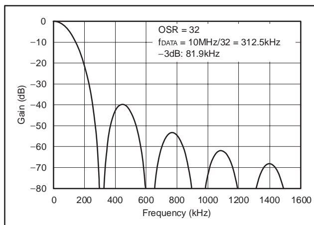
Figure 9. Frequency Response of Sinc 3 Filter
