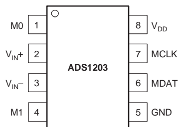
TSSOP PACKAGE (TOP VIEW)
