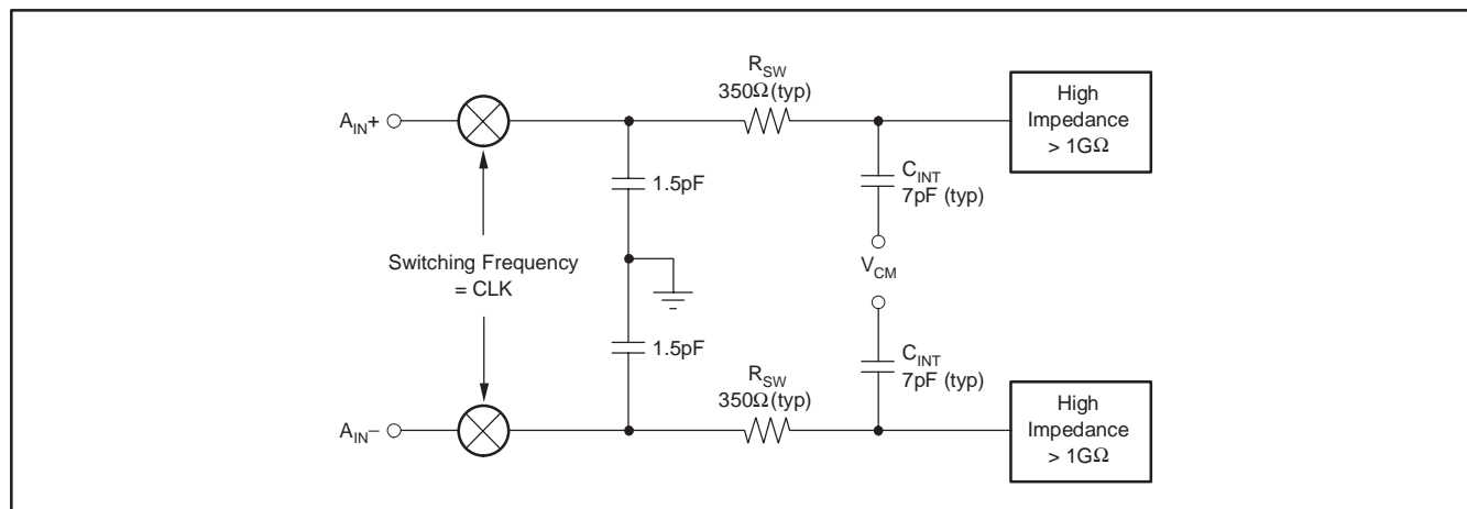
Figure 6. Input Impedance of the ADS1203
