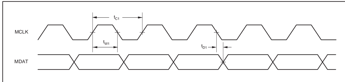
Figure 1. Mode 0 Operation
