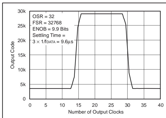
Figure 10. Pulse Response of Sinc 3 Filter ( f_{MOD} = 10\text{MHz} )
