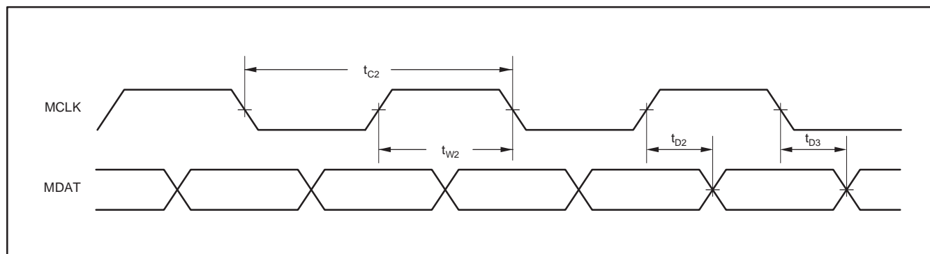
Figure 2. Mode 1 Operation
