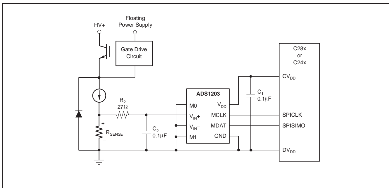
Figure 15. Application Diagram without Galvanic Isolation in Mode 0
