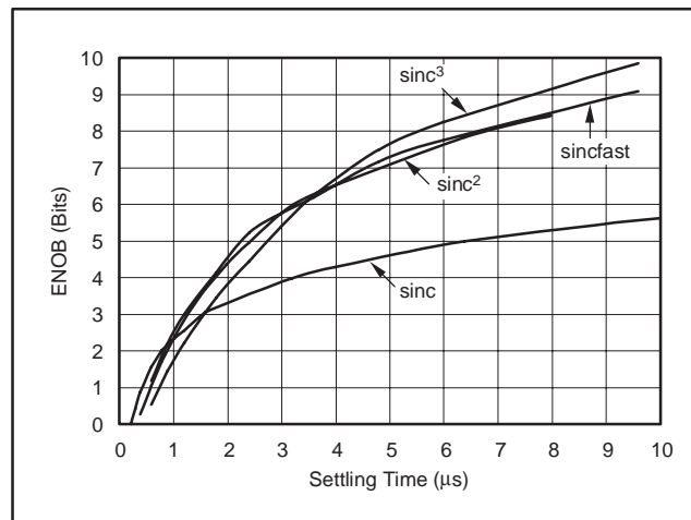
Figure 12. Measured ENOB vs Settling Time
