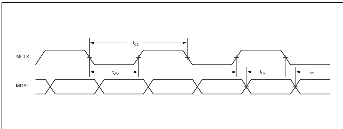
DIAGRAM 2: Mode 1 Operation.
