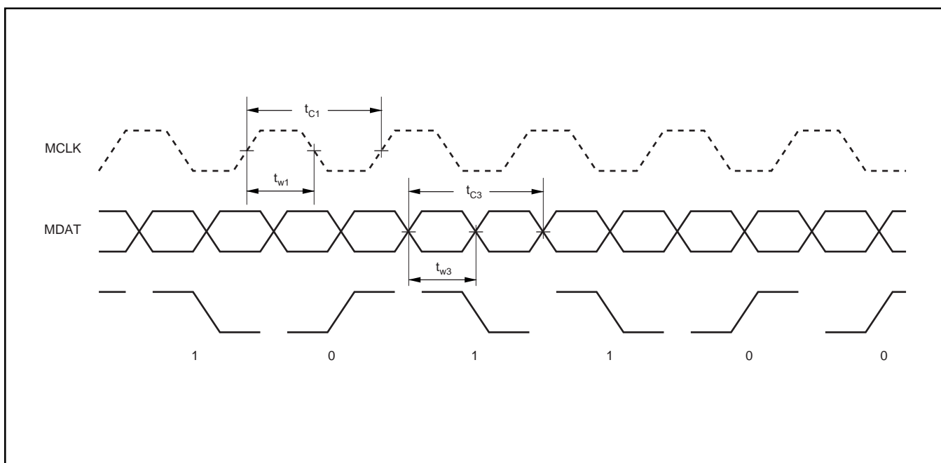
DIAGRAM 3: Mode 2 Operation.
