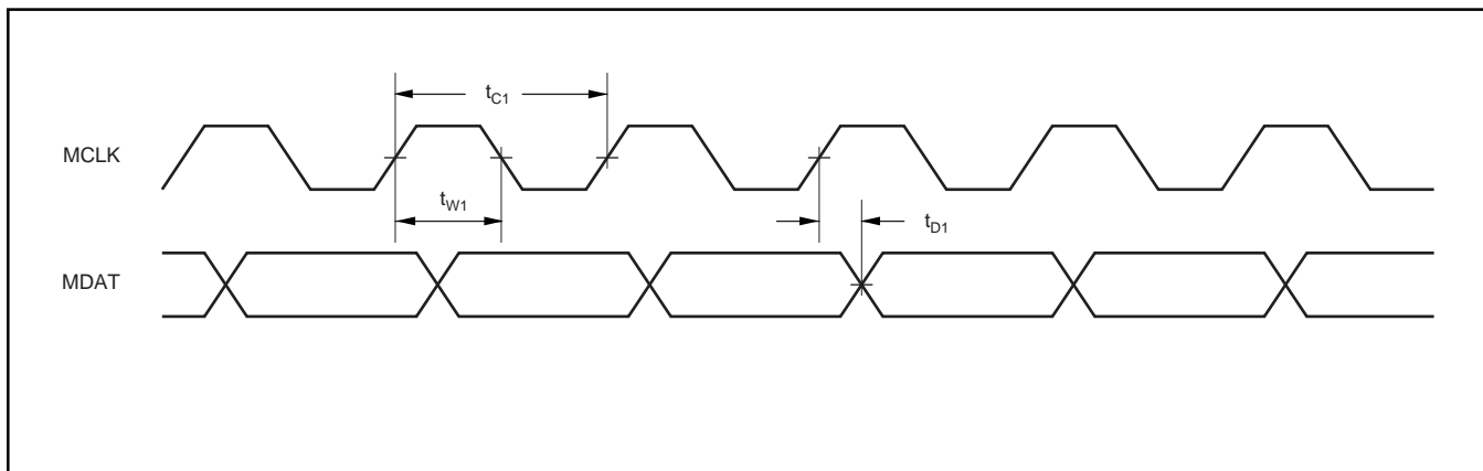
DIAGRAM 1: Mode 0 Operation.
