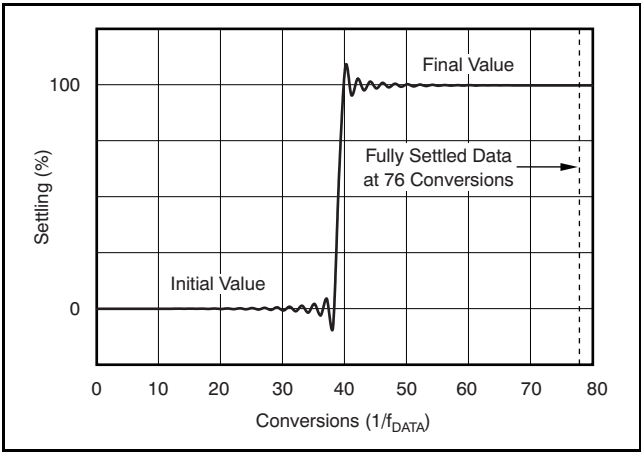
Figure 6. Step Response
