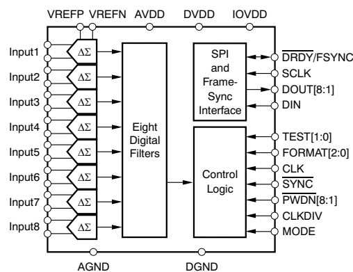
ADS1178
