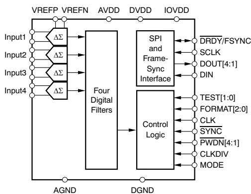
ADS1174
