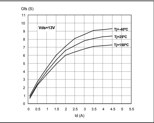
Figure 14. Transconductance
