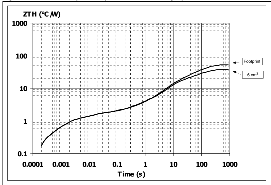
Figure 27. Thermal impedance junction ambient single pulse
