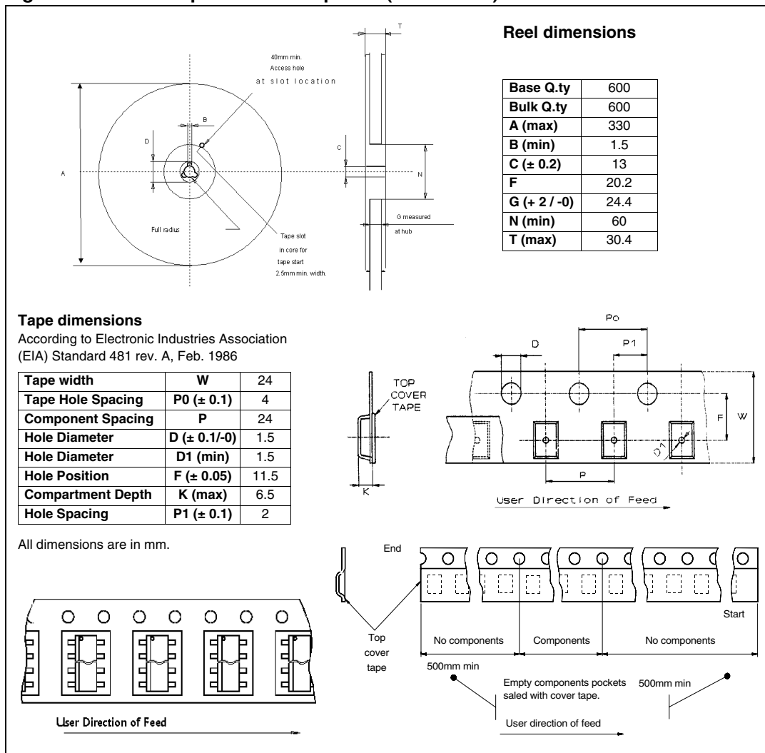
Figure 32. SO-28 tape and reel shipment (suffix “TR”)
