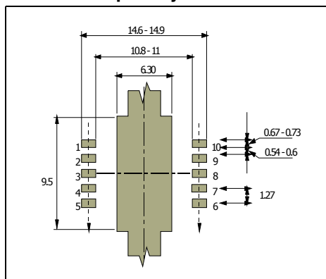
Figure 30. PowerSO-1 pad layout
