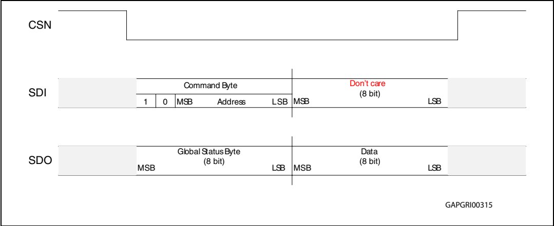
Figure 14. SPI read and clear operation
