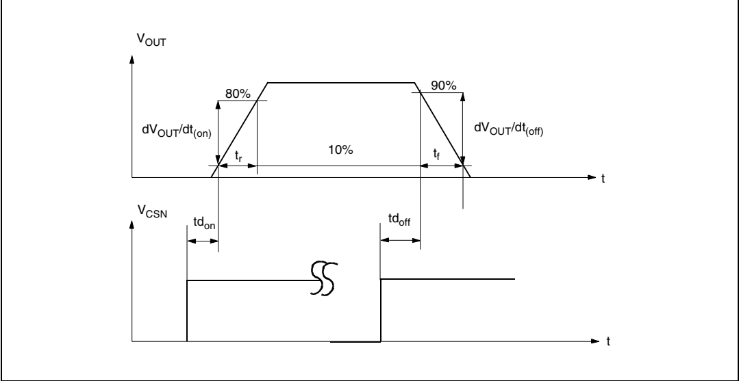
Figure 22. Switching characteristics
