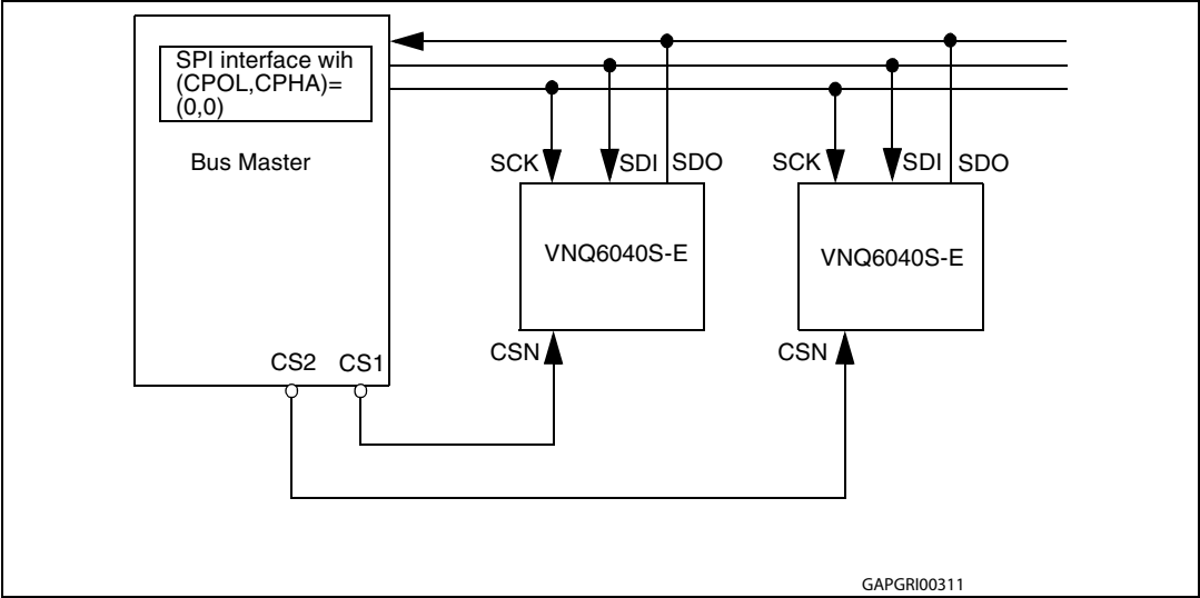
Figure 11. Supported SPI mode
