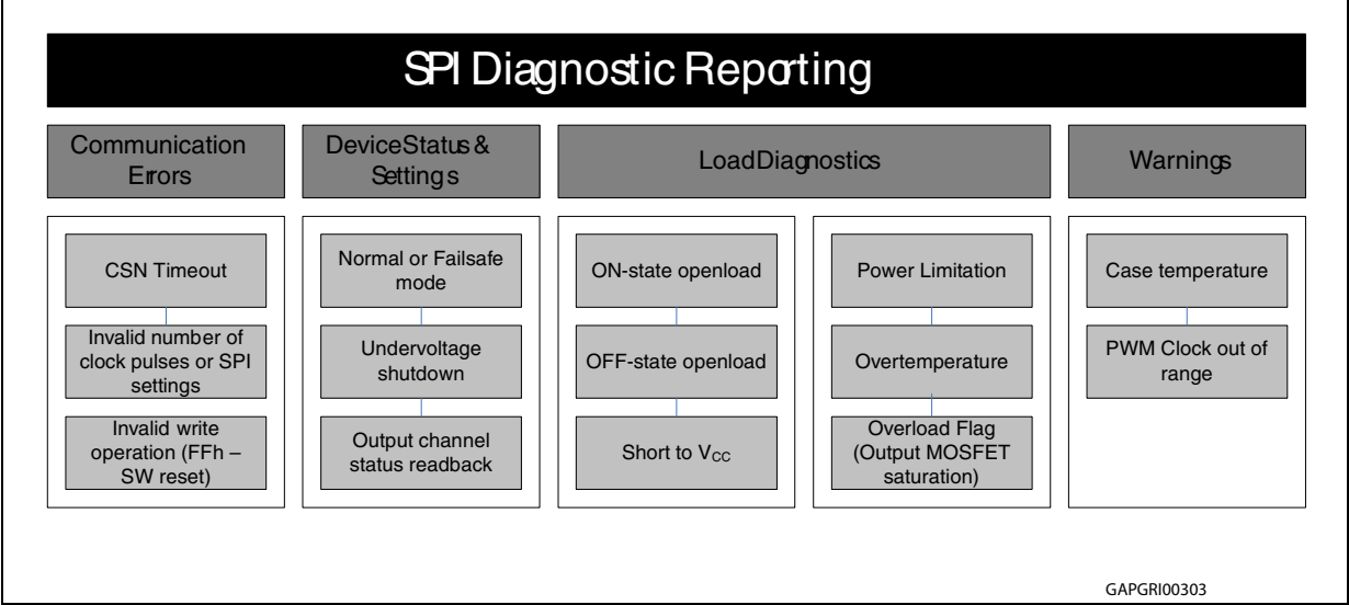
Figure 2. SPI diagnostic reporting
