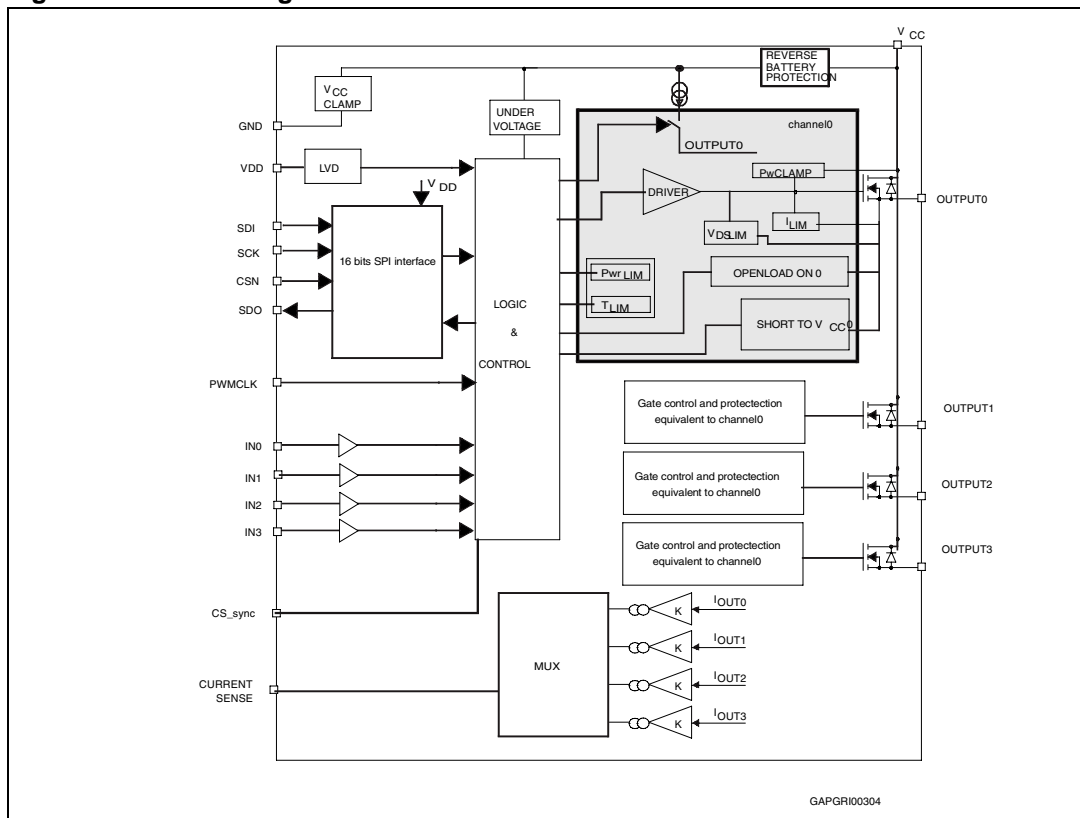
Figure 3. Block diagram
