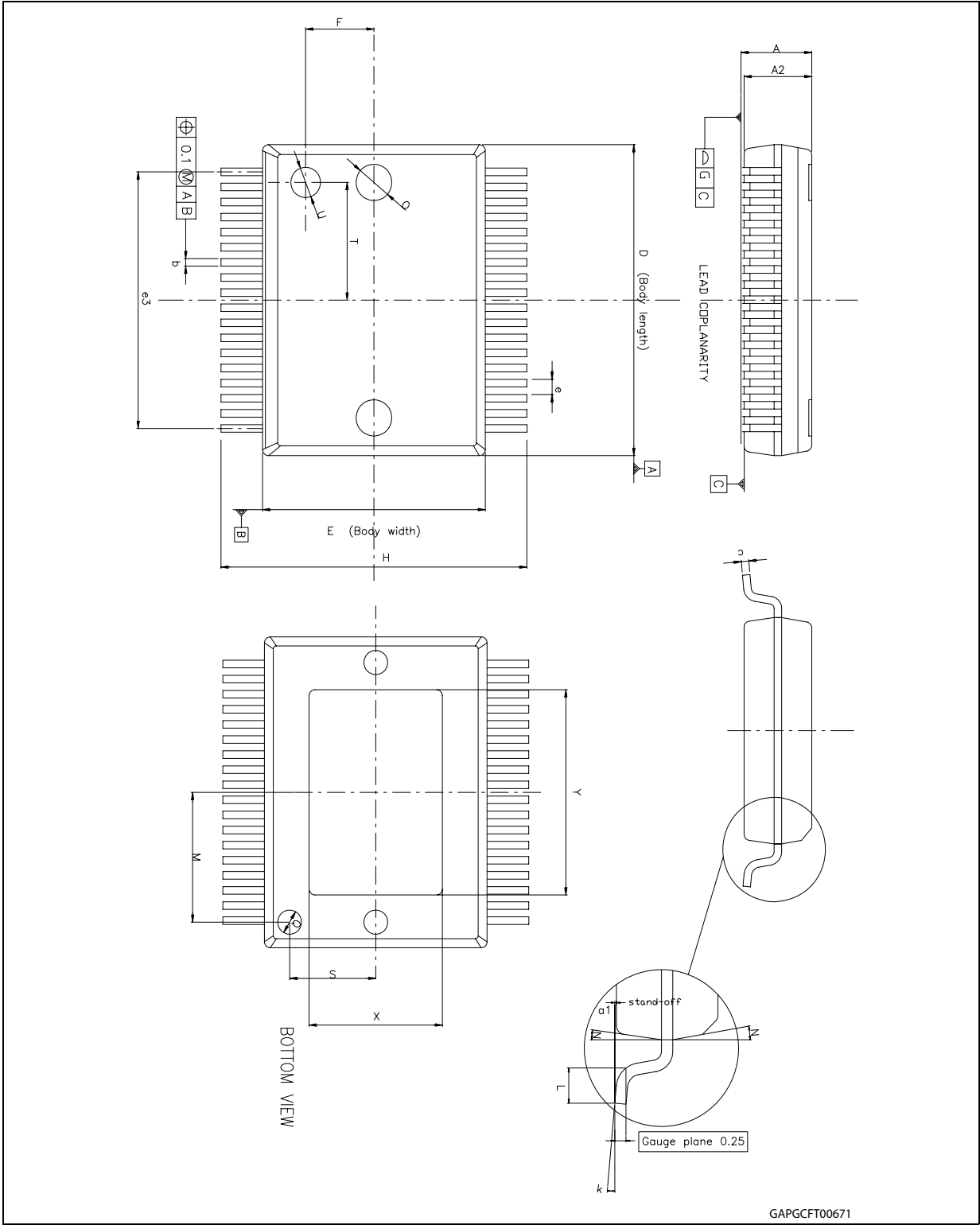
Figure 31. PowerSSO-36 package dimensions
