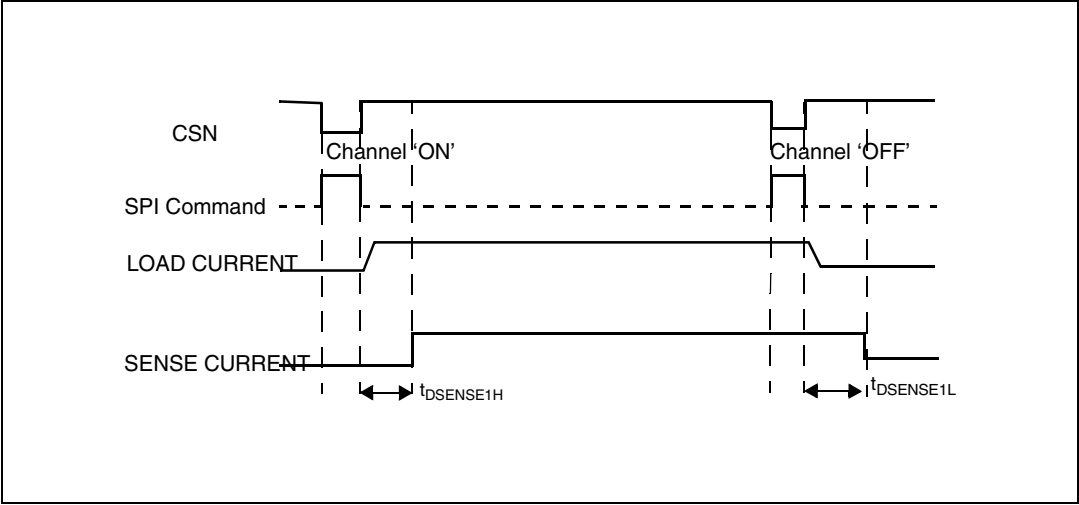
Figure 22. Switching characteristics
