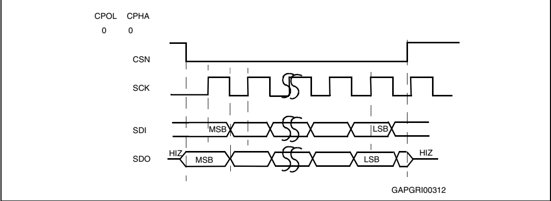
Figure 11. Supported SPI mode
