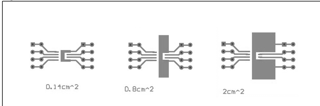
Figure 34. SO-8 PC board
