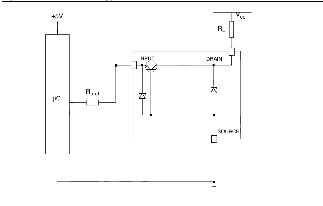
Figure 7. VNL5090N3-E application schematic
