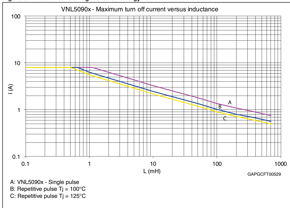
Figure 9. Maximum demagnetization energy (1)
