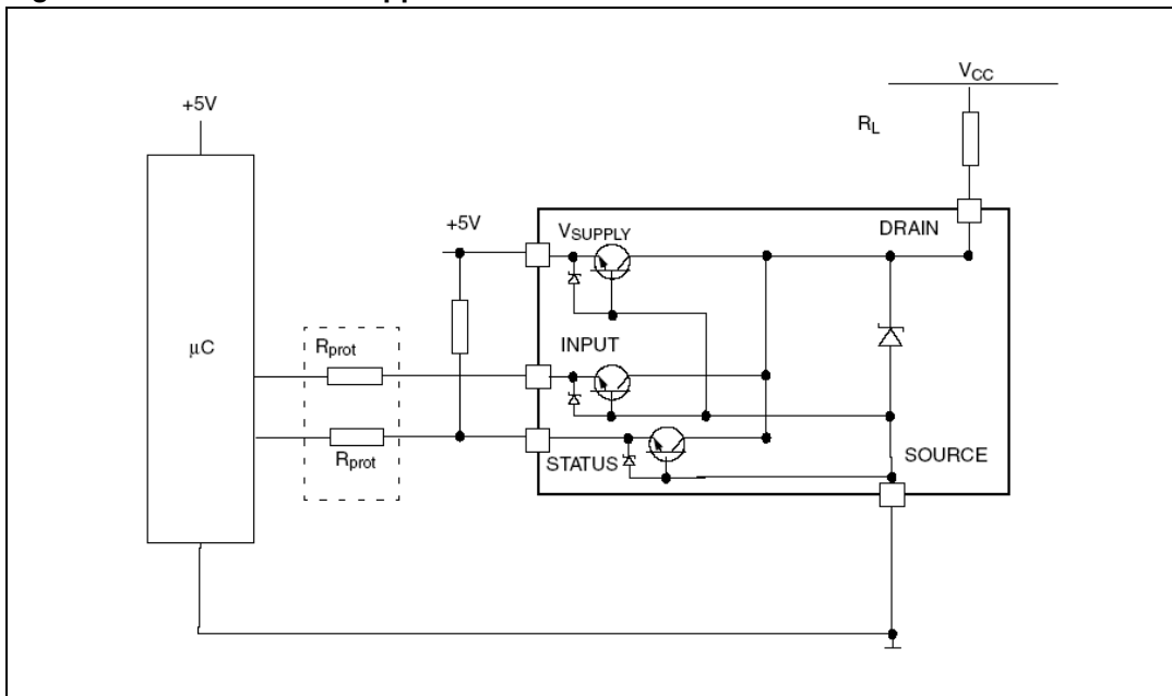
Figure 8. VNL5090S5-E application schematic
