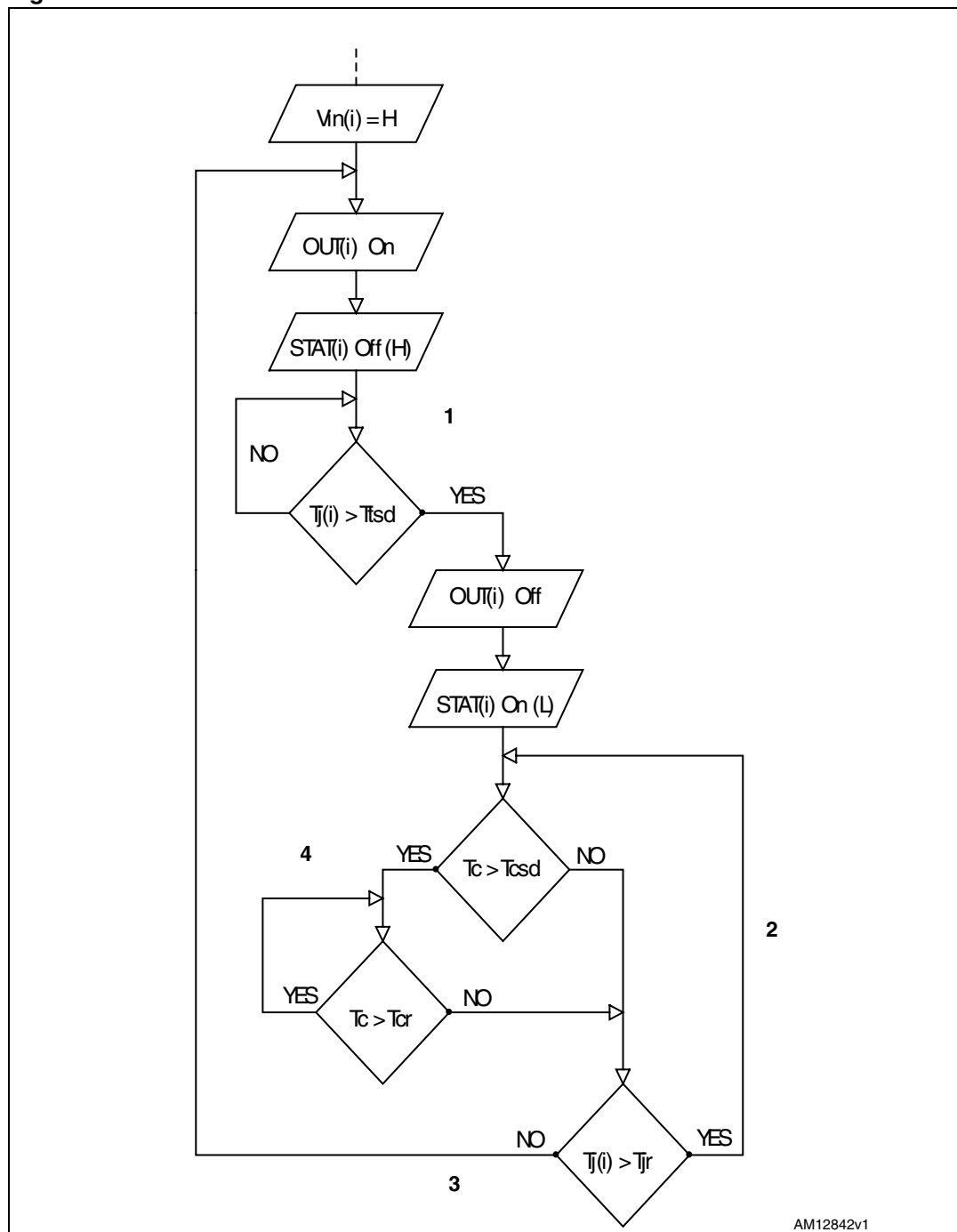
Figure 12. Thermal behavior
