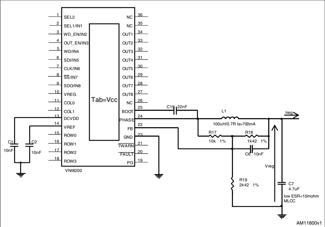
Figure 9. Typical circuit for switching regulation V_{DC-out} = 5\text{ V}
