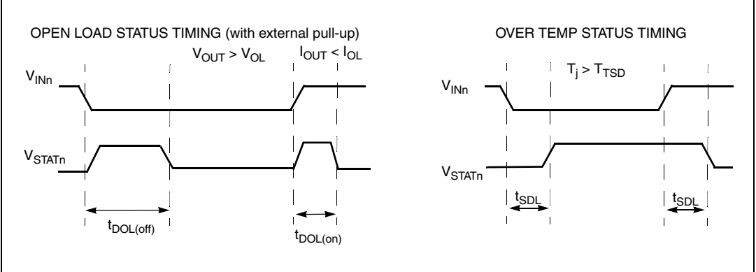
Figure 4. Status timings
