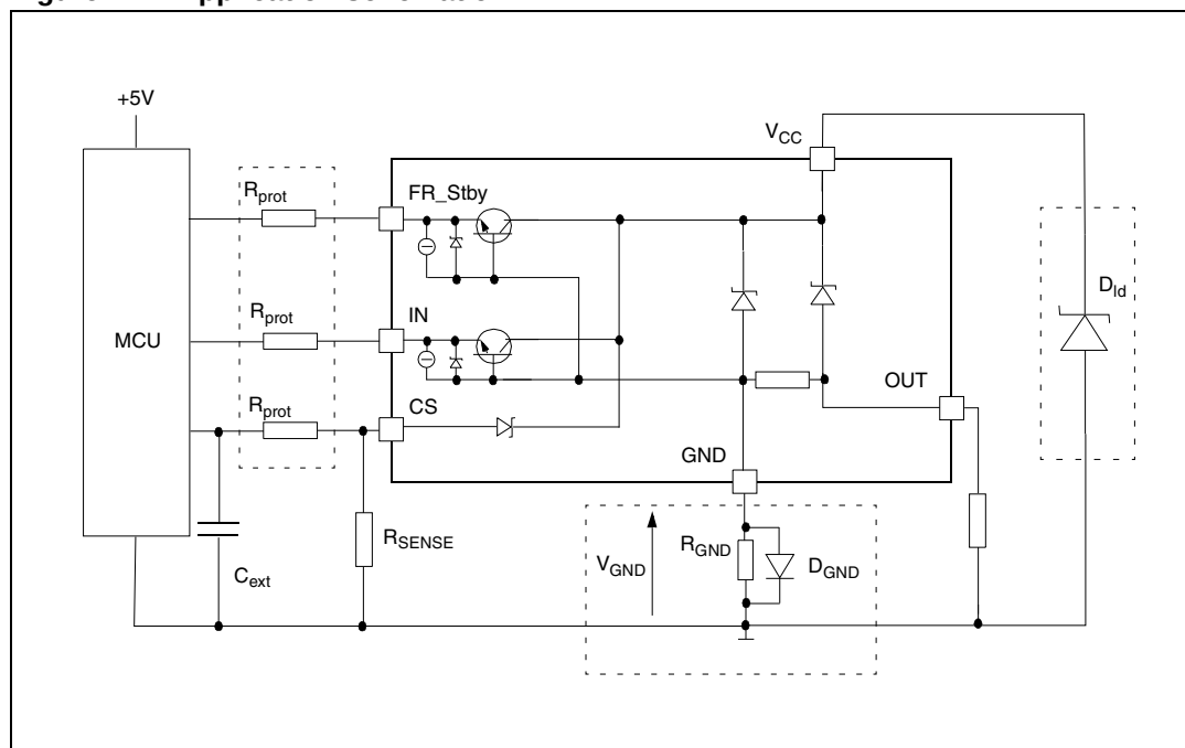
Figure 24. Application schematic
