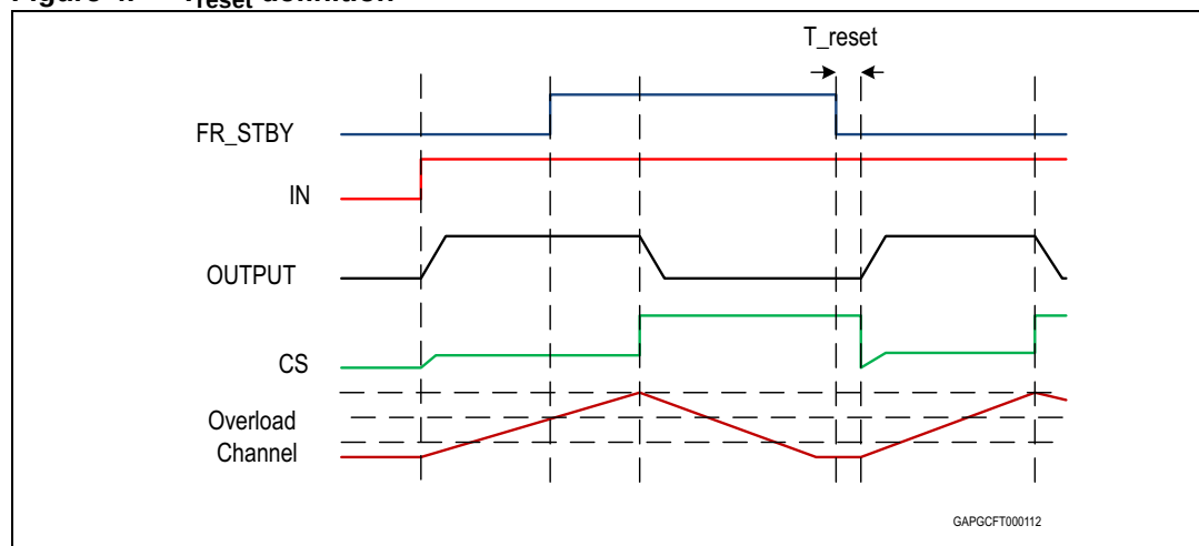
Figure 4. T_{reset} definition
