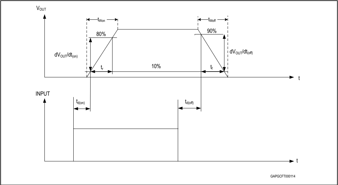
Figure 8. Switching characteristics
