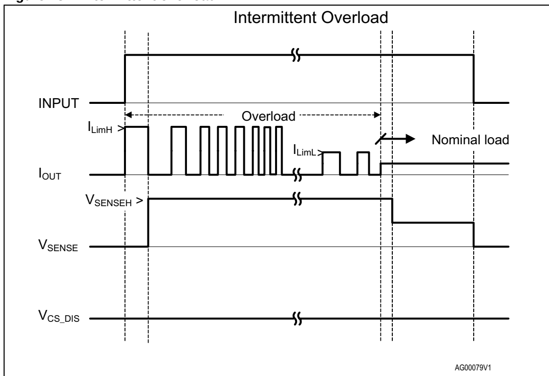
Figure 13. Intermittent overload
