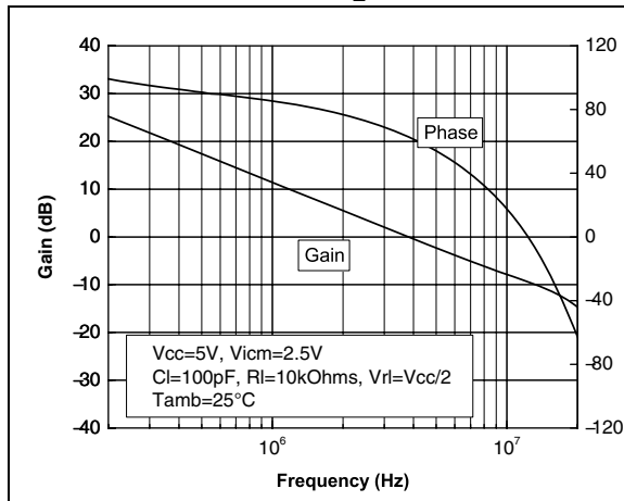
Figure 3. Voltage gain and phase vs. frequency, C_L = 100 pF
