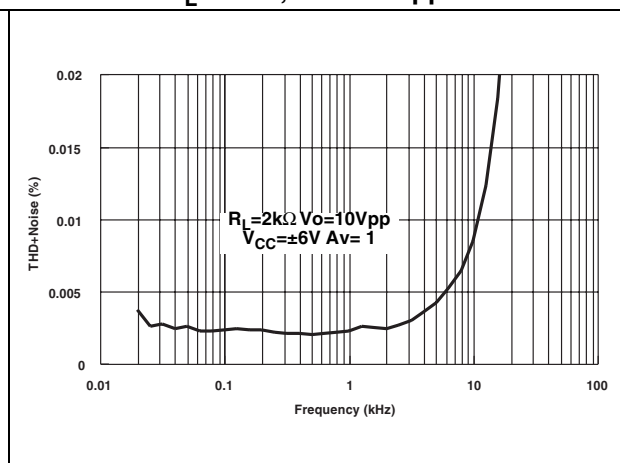
Figure 6. THD + noise vs. frequency, R_L = 2 k \Omega , V_o = 10 Vpp
