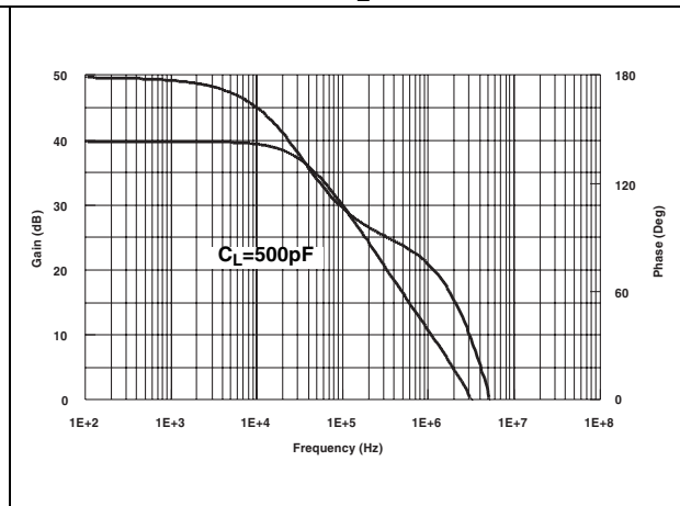
Figure 4. Voltage gain and phase vs. frequency, C_L = 500 pF
