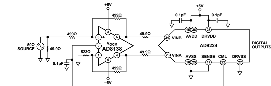
Figure 46. AD8138 Driving an AD9224, a 12-Bit, 40 MSPS ADC
