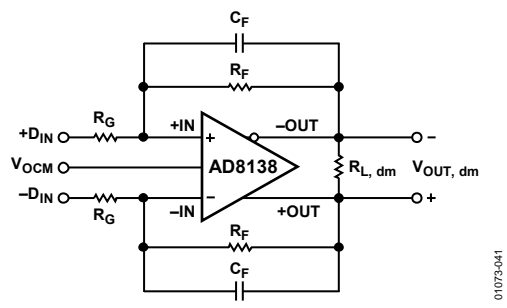
Figure 42. Circuit Definitions
