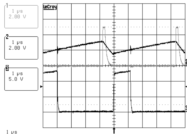
Figure 13 TYPICAL WAVEFORMS
