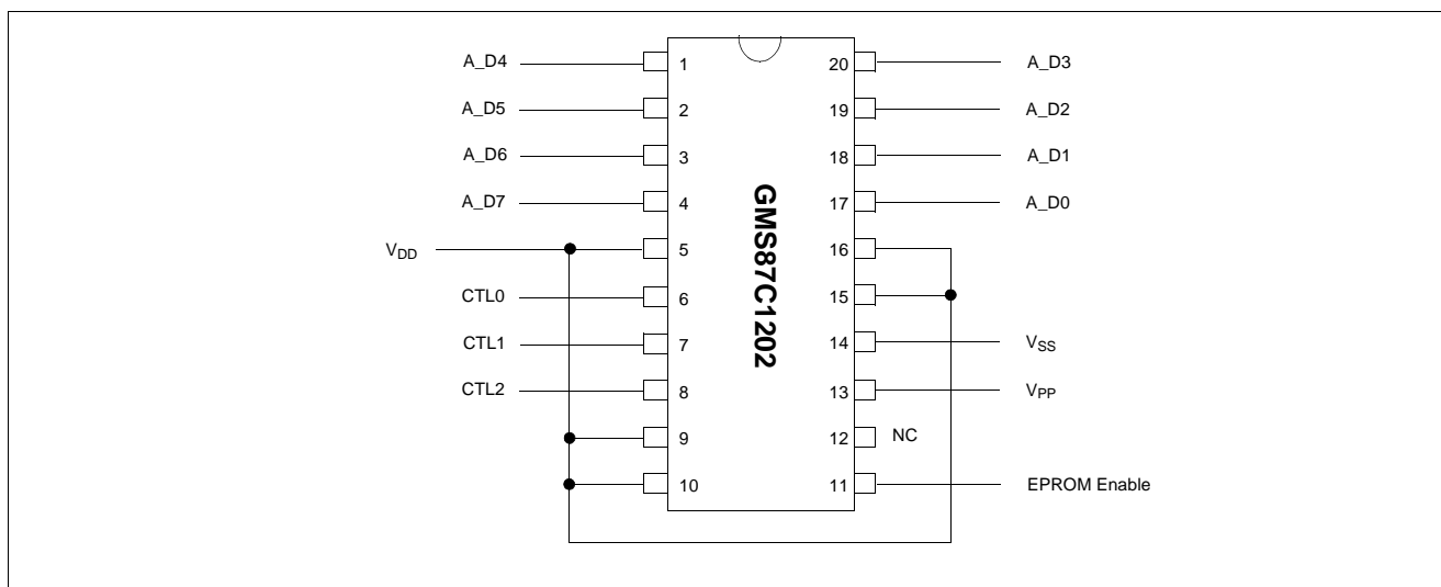
Figure 23-3 Pin Assignment
