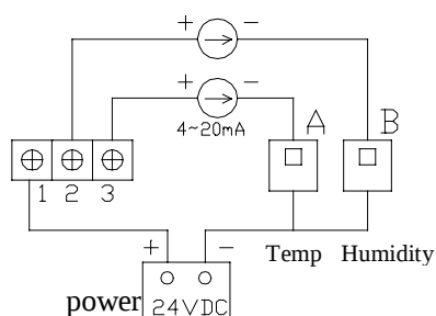
4-20mA output
