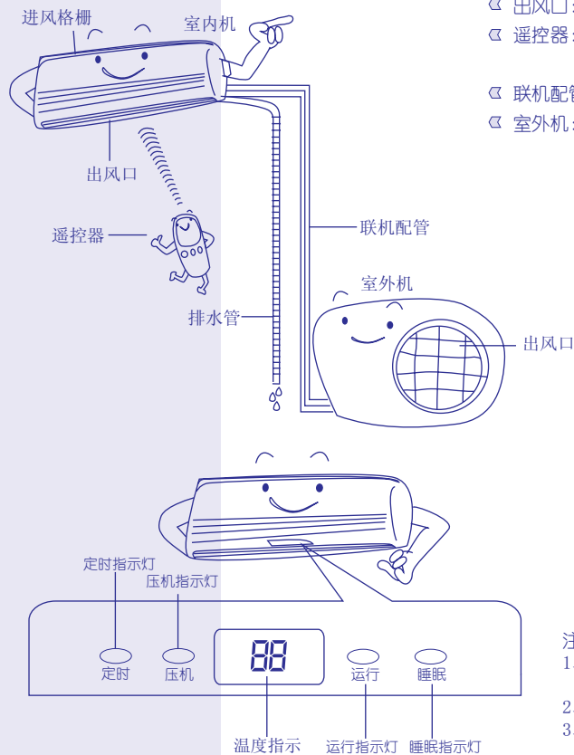
Composition of the air conditioner 空调组成
