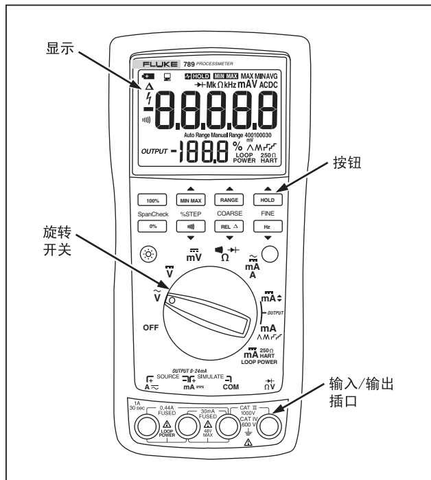
图 1. Fluke 789 ProcessMeter
