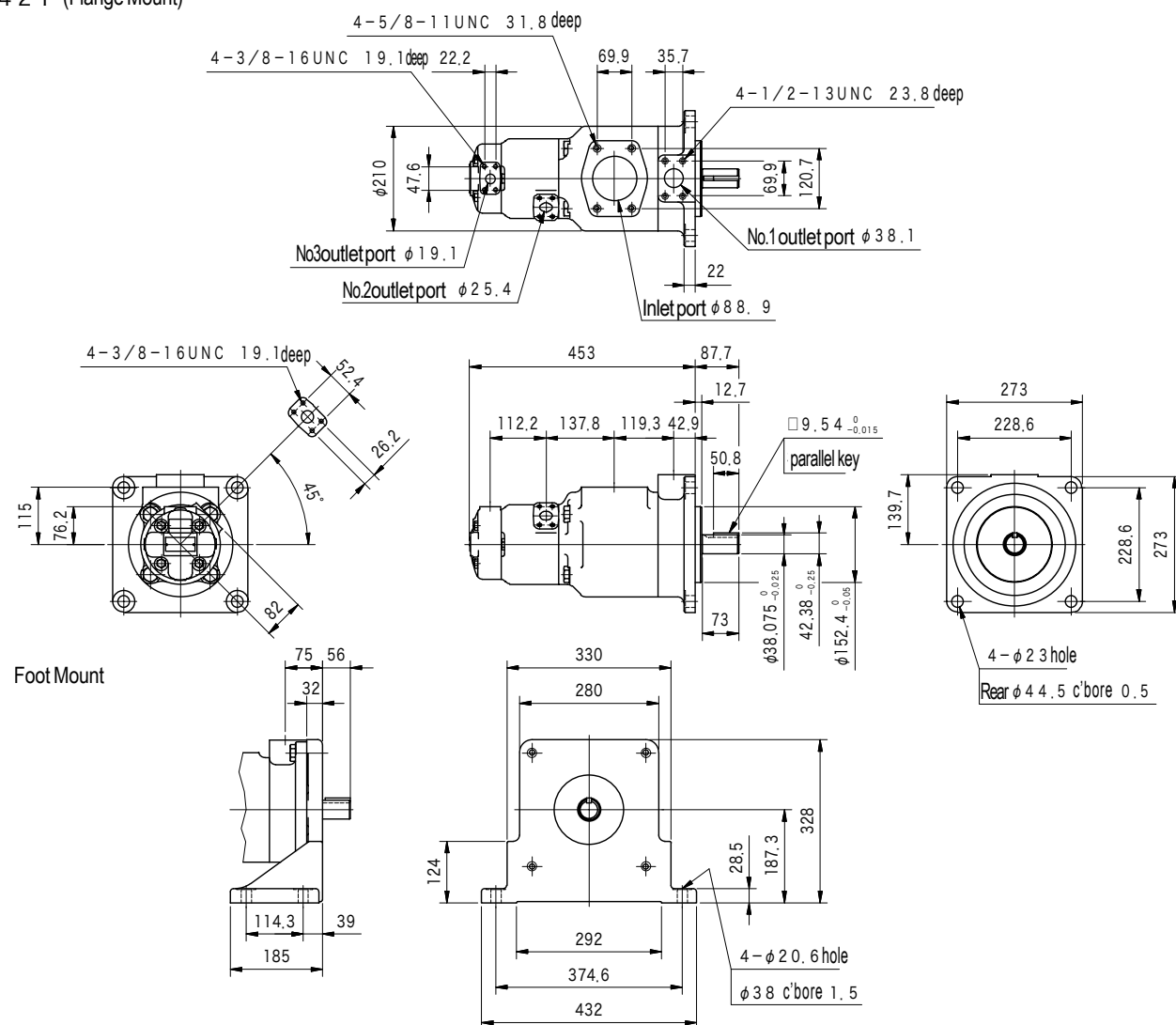
S Q P 4 2 1 (Flange Mount)
