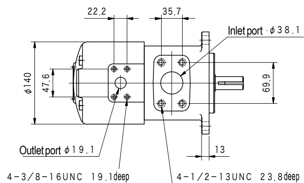
S Q P S 1 (Flange Mount)
