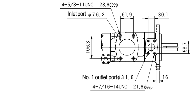
3520VQ (Flange Mount)
