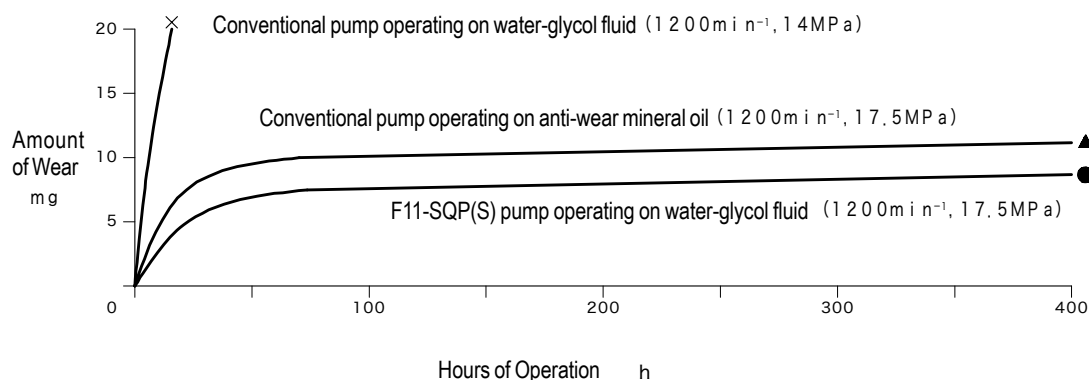
Vane Wear Comparison (Tokimec pumps)
