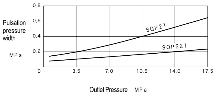
•Comparison of Pump Pressure Pulsations
