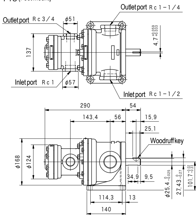
V-129, 139, 149 (Flange Mount)
