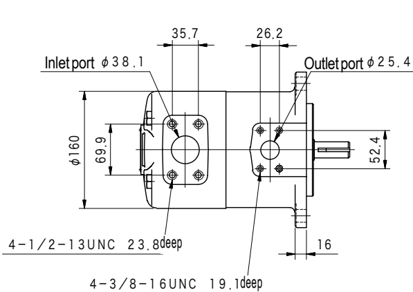
S Q P S 2 (Flange Mount)
