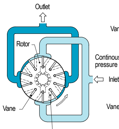
Fig.1 Pressure acts below vanes to push vane tips against the cam ring and provides optimum sealing of vane chambers.
