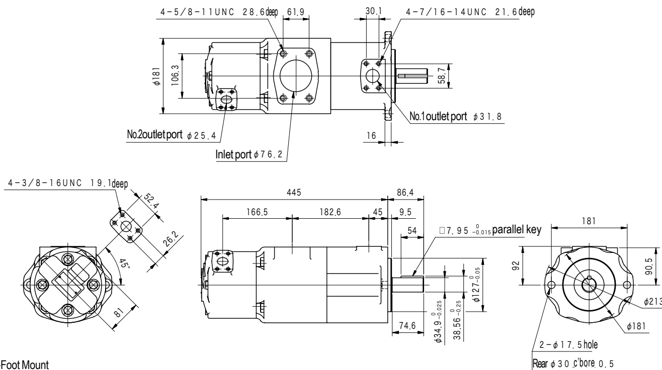
S Q P S 3 2 (Flange Mount)
