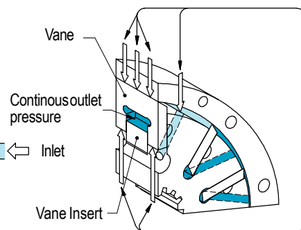
Fig.2 Shaft rotation causes alternate quadrant shifts in delivery load pressure and inlet suction pressures.
