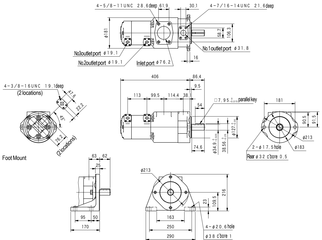
SQP 311 (Flange Mount)
