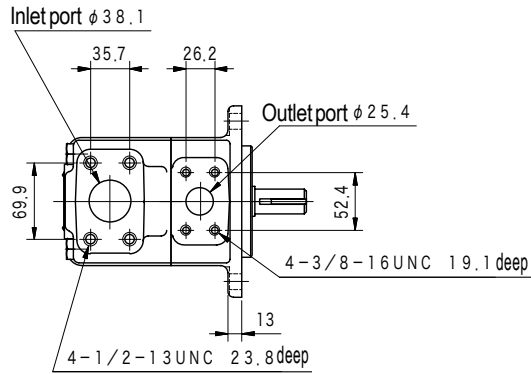
2 5 V Q (Flange Mount)
