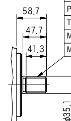
No.11 Spline Shaft End
