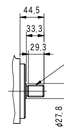
No.11 Spline Shaft End
