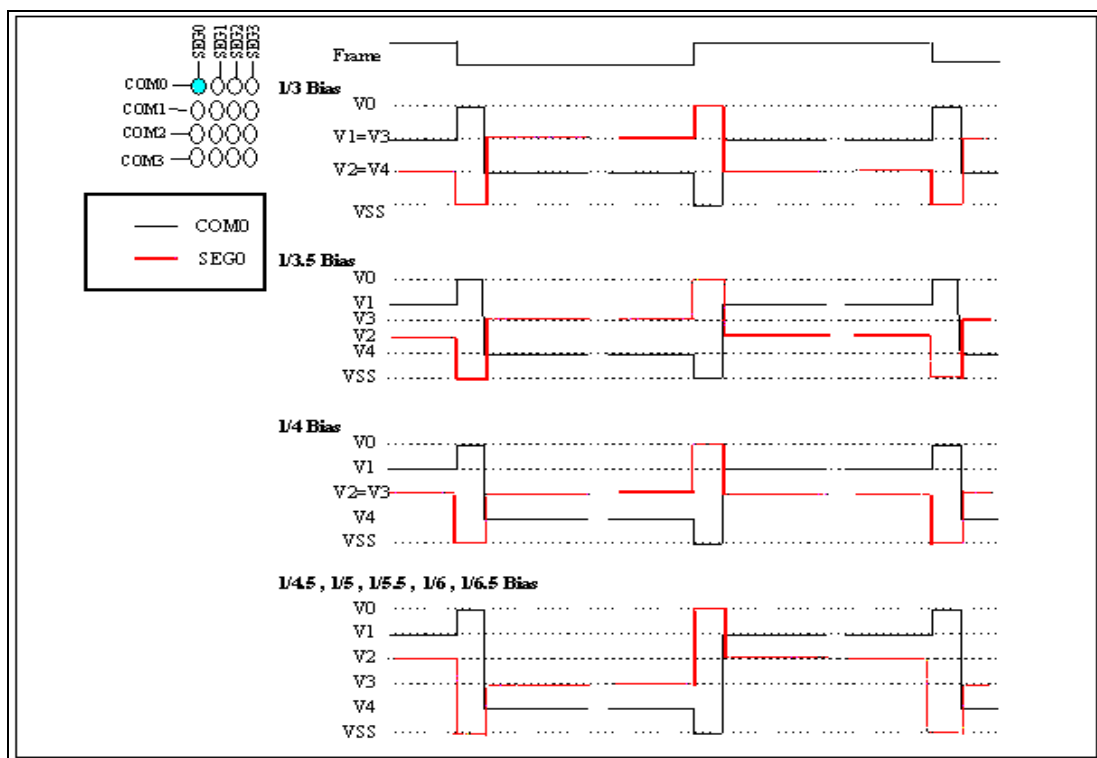
Figure 8-23b LCD Waveform
