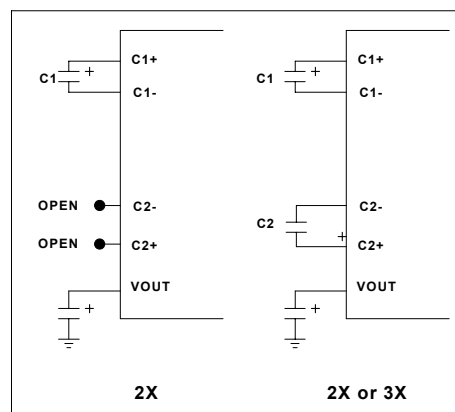
Figure 8-22 Voltage Converter External Capacitors
