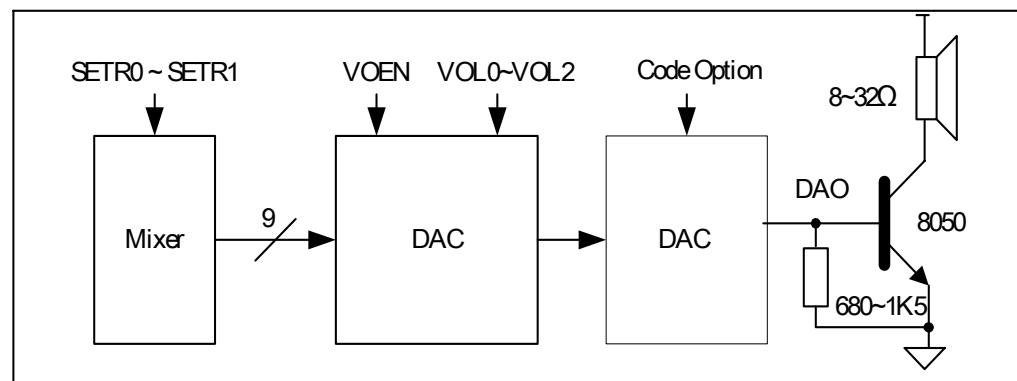
Figure 8-28 DAC Function Block Diagram
