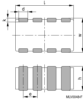
4-fold array
