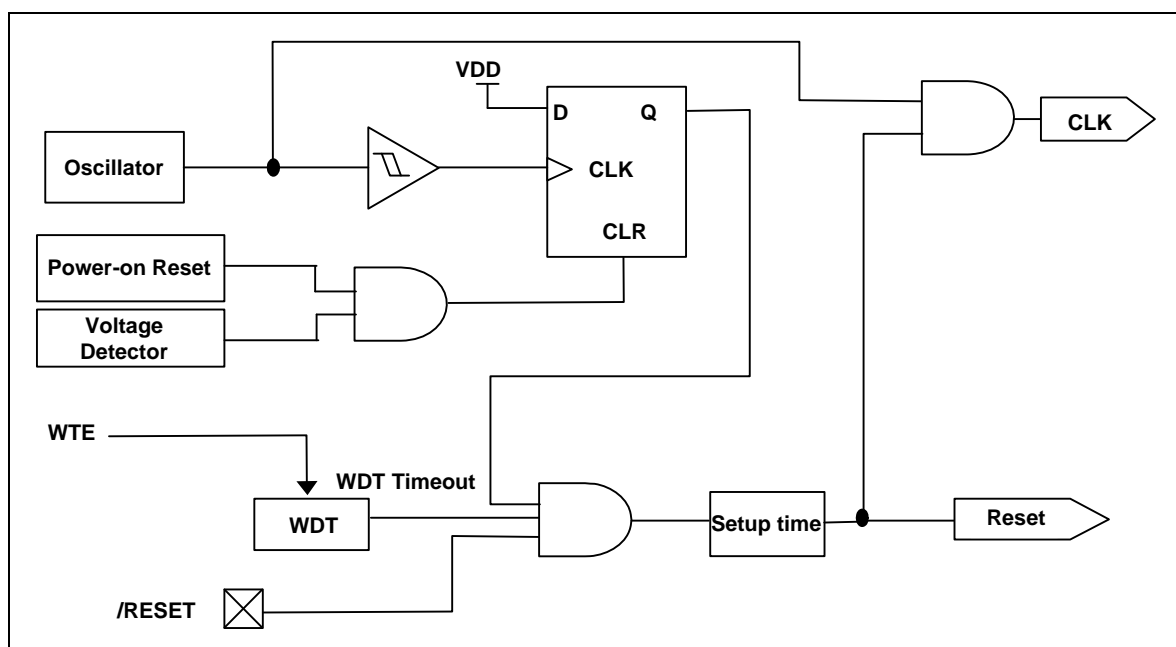
Figure 6-18 Controller Reset Block Diagram
