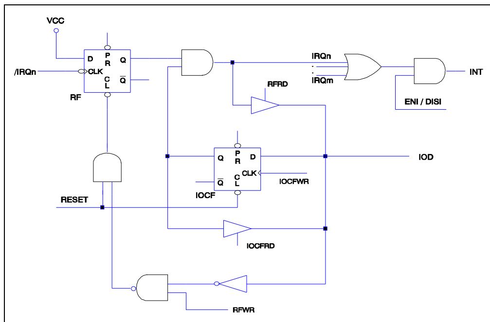
Figure 6-19 Interrupt Input Circuit
