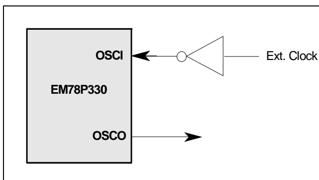
Figure 6-26 External Clock Input Circuit
