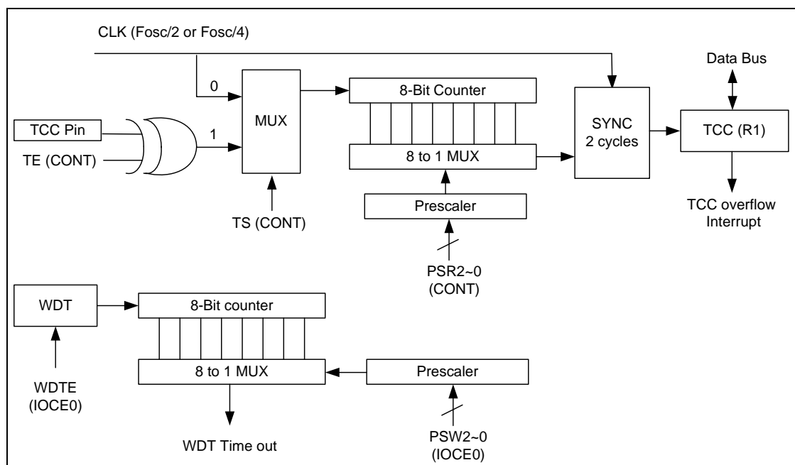
Figure 6-5 TCC and WDT Block Diagram
