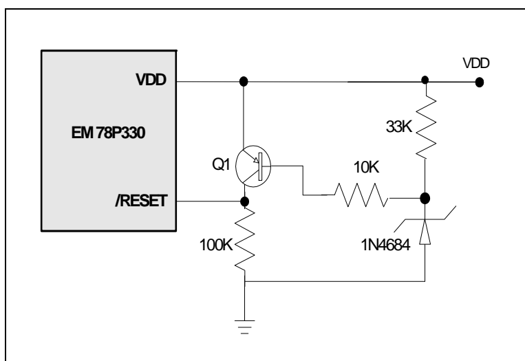
Figure 6-30 Residual Voltage Protection Circuit 1
