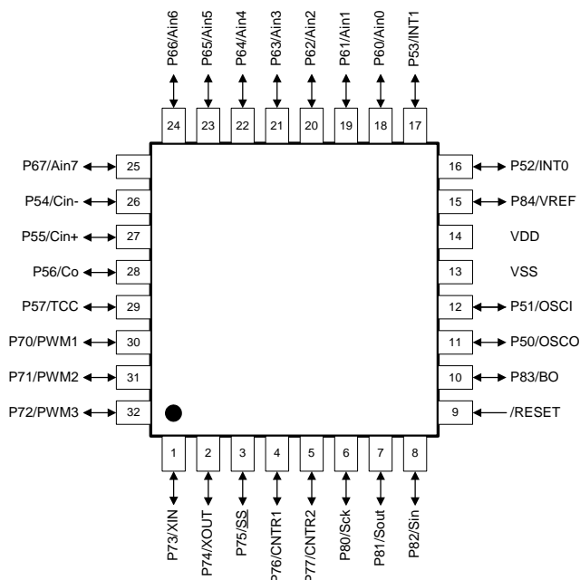
Figure 3-2 EM78P331NQS/J
