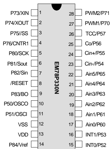
Figure 3-1 EM78P330NPS/NAKS/NMS/J
