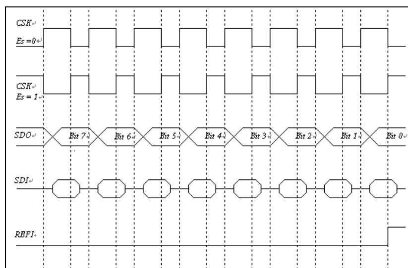
Figure 6-15 SPI Mode with /SS Disabled
