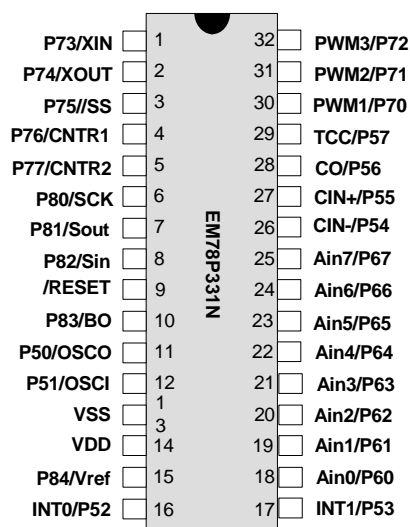
Figure 3-3 EM78P331NKS/NPS/NMS/J
