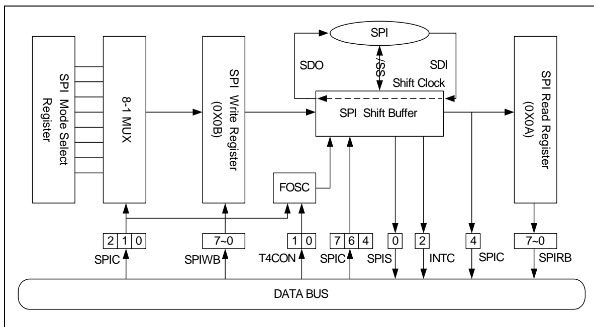
Figure 6-14 SPI Transmission Function Block Diagram
