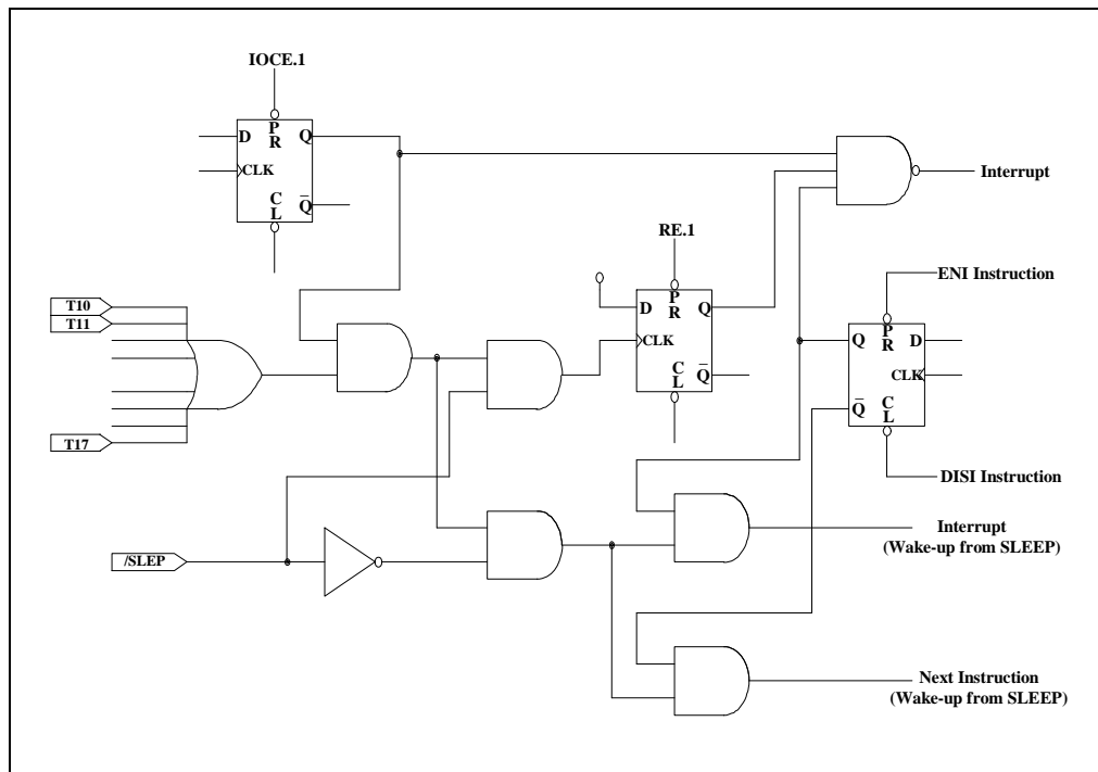
Figure 6-9 Port 6 Block Diagram with Input Change Interrupt/Wake-up
