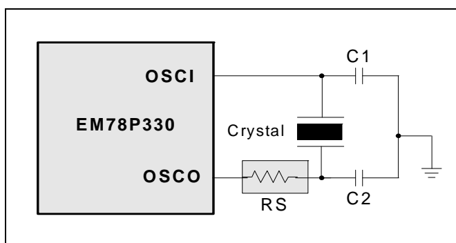
Figure 6-27 Crystal/Resonator Circuit
