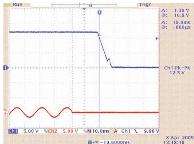
Figure 3 Hold up example at 45 W load with 115 VAC input (17.2ms)
