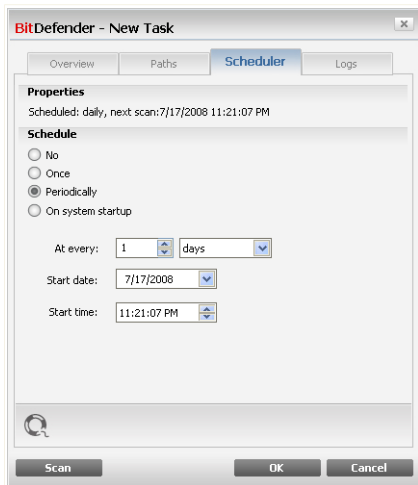
Scheduler
