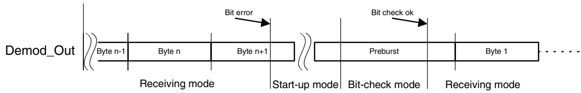
Figure 48. Bit Error (TMODE = 0)
