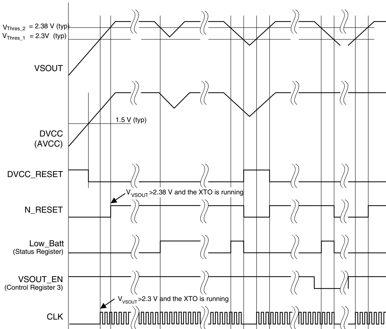
Figure 23. Reset Timing
