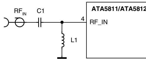
Figure 7. Input Matching to 50 \Omega
