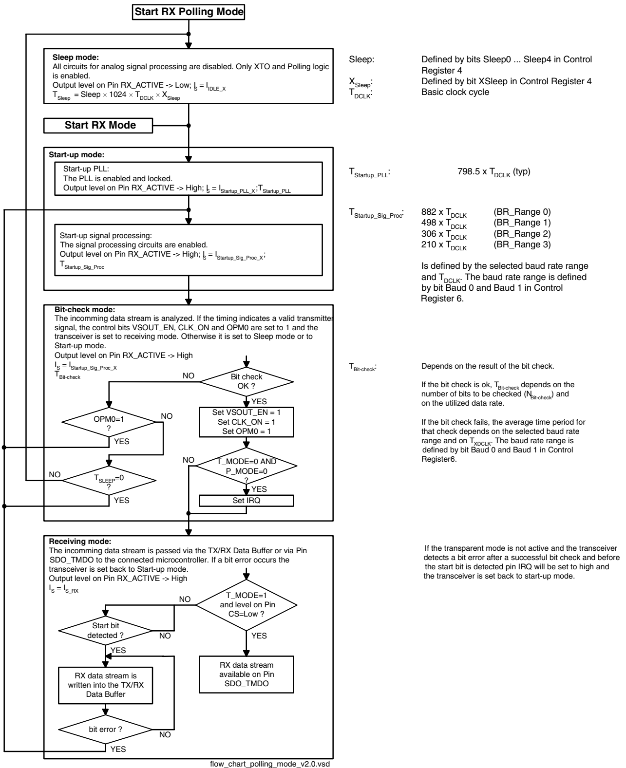
Figure 40. Flow Chart RX Polling Mode/RX Mode
