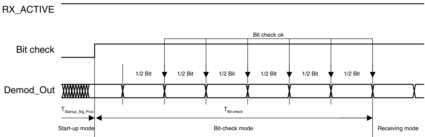
Figure 41. Timing Diagram for Complete Successful Bit-check (Number of checked Bits: 3)
