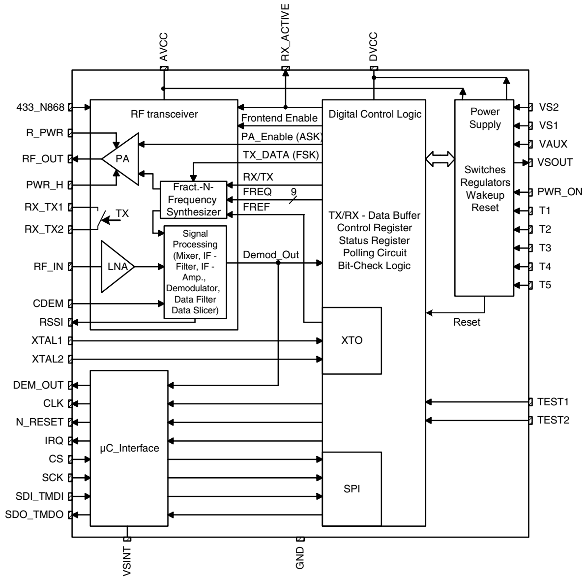
Figure 3. Block Diagram
