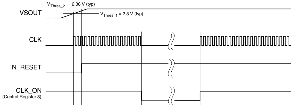
Figure 20. Clock Timing
