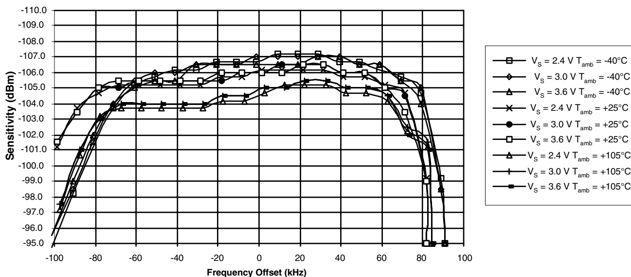
Figure 8. Measured Sensitivity 433.92 MHz/FSK/20 kBaud/ \pm 16 kHz/Manchester versus Frequency Offset, Temperature and Supply Voltage
