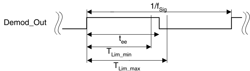
Figure 42. Valid Time Window for Bit-check
