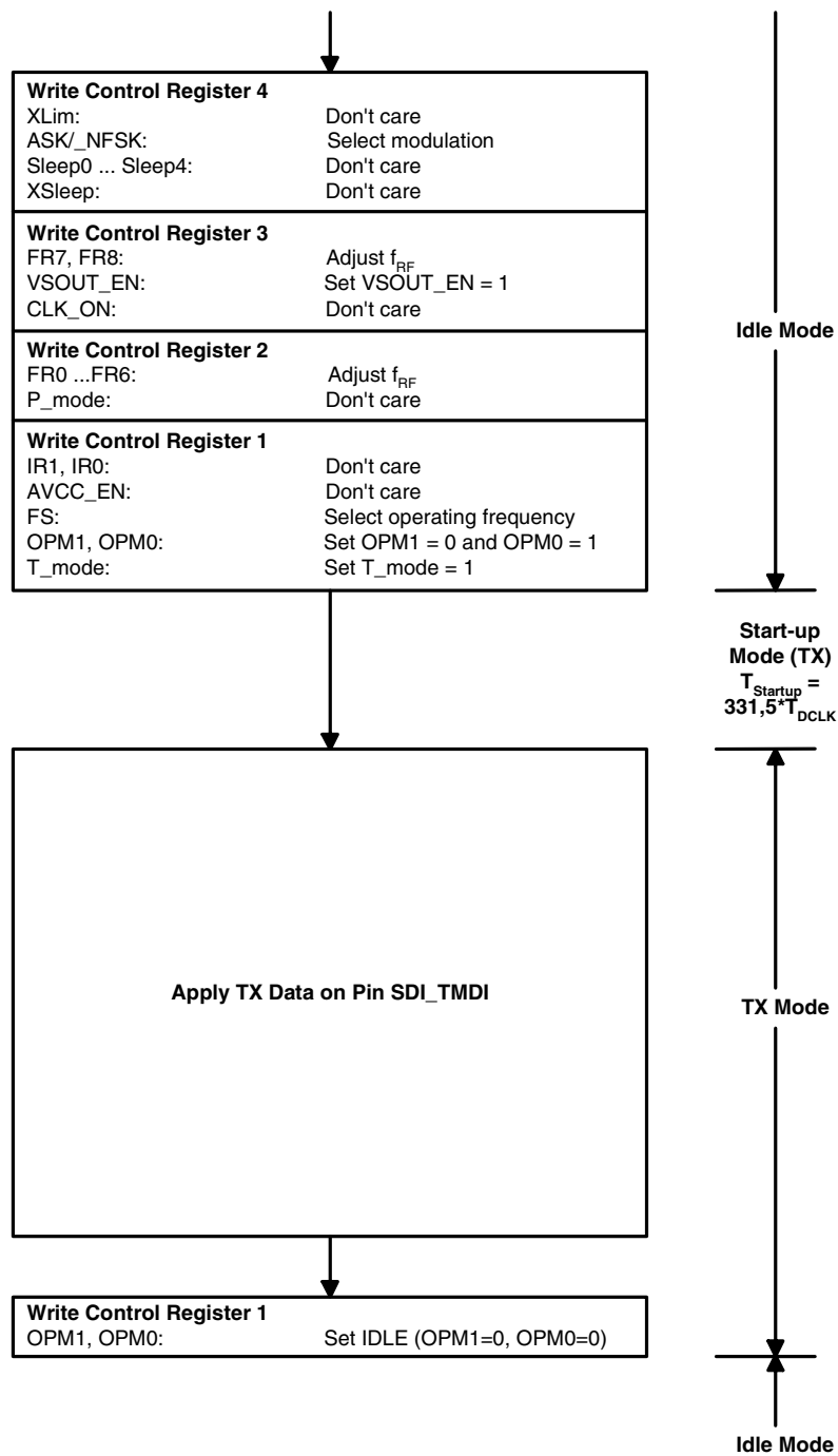
Figure 50. TX Transparent Mode (T_MODE = 1)
