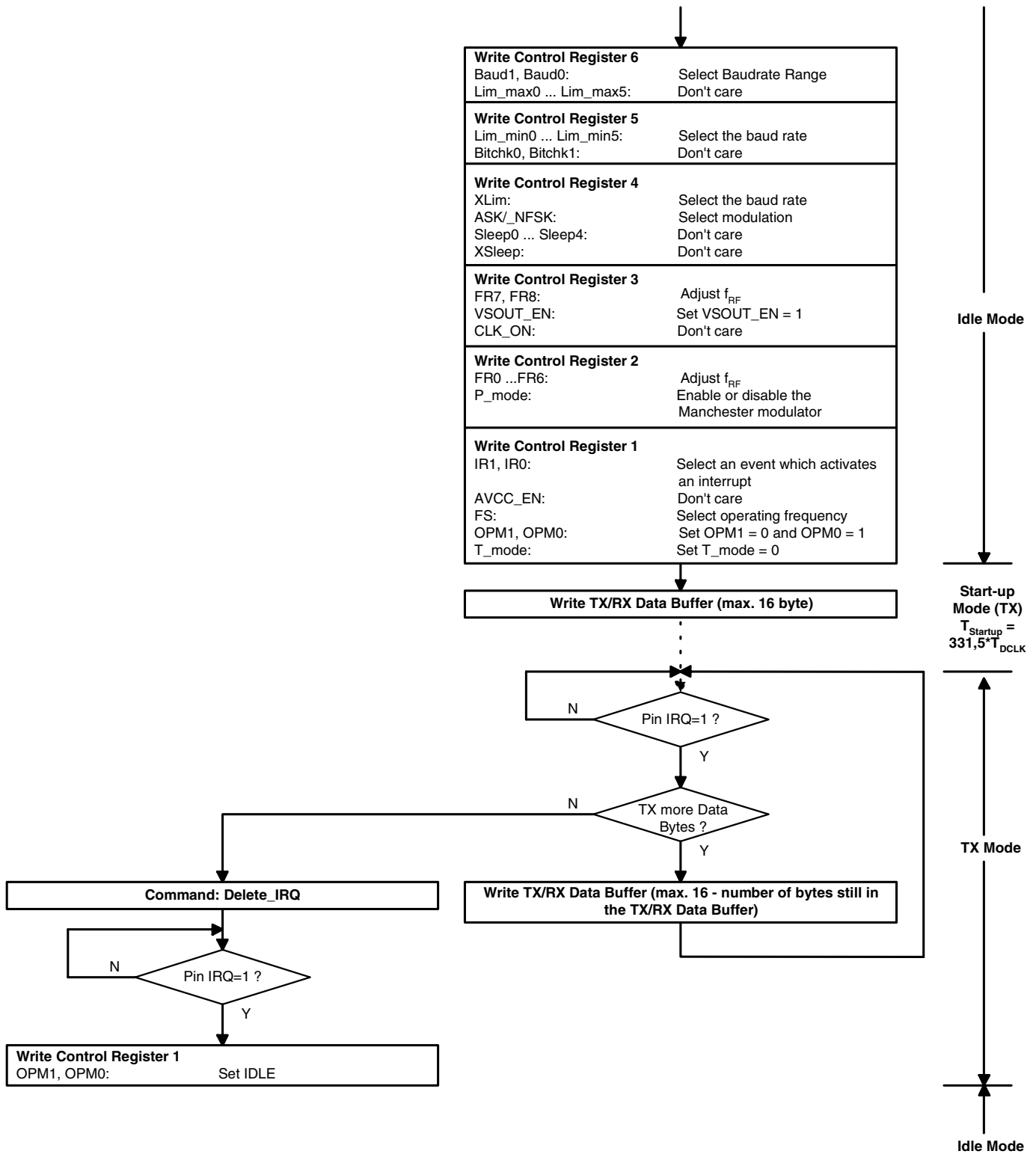
Figure 49. TX Operation (T_MODE = 0)
