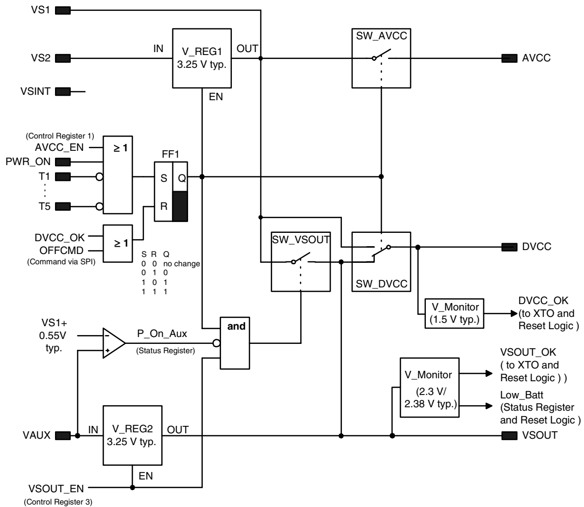
Figure 21. Power Supply
