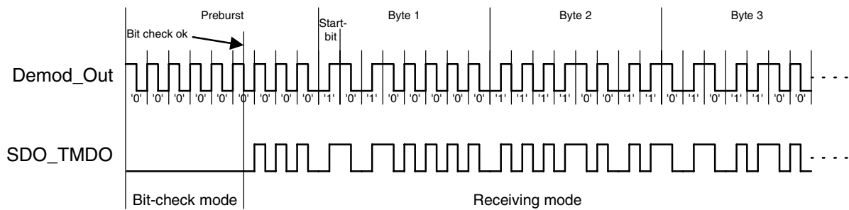
Figure 46. Receiving Mode ( \text{TMODE} = 1 )
