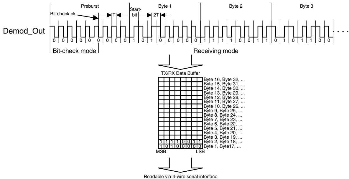
Figure 47. Receiving Mode (TMODE = 0)
