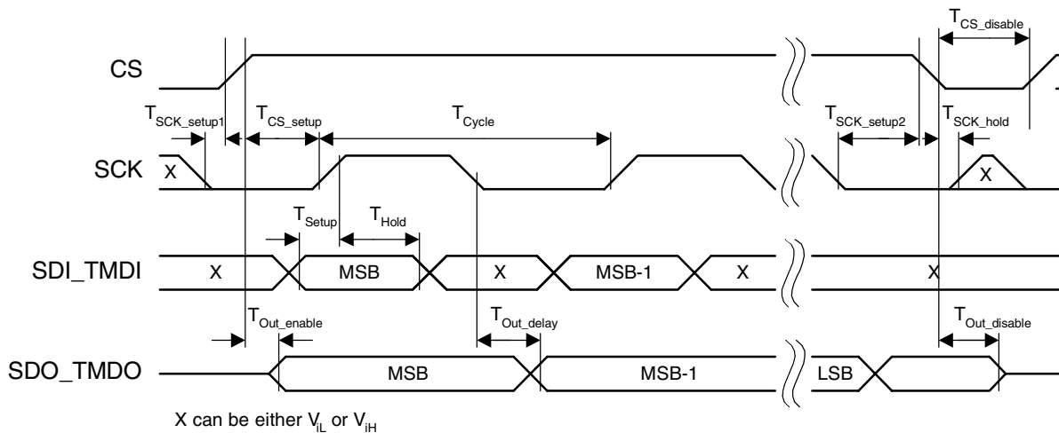
Figure 39. Serial Timing
