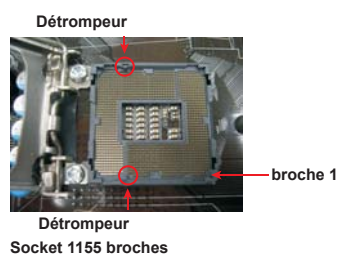
Socket 1155 broches
