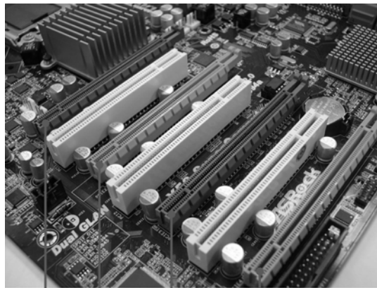
PCIe1 slot (x16 or x8 mode)
