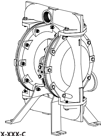
66615X-XXX-C 1-1/2" 隔膜泵
