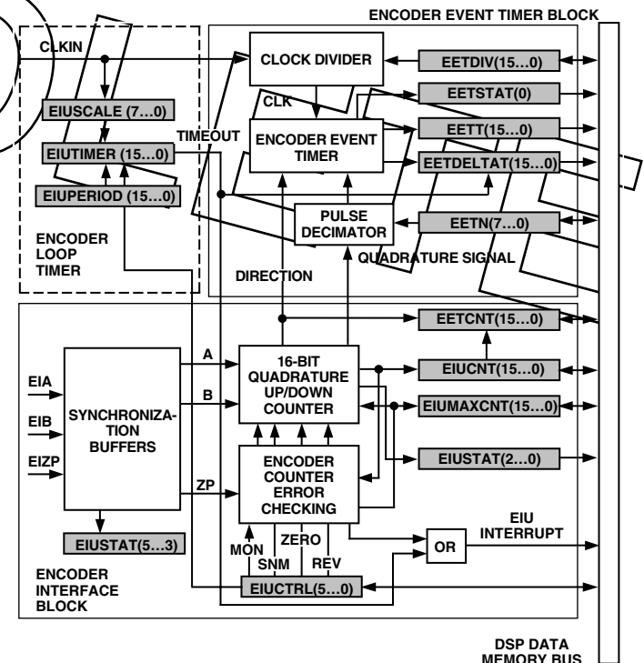
Figure 16. Configuration of Encoder Interface System of ADCM300
