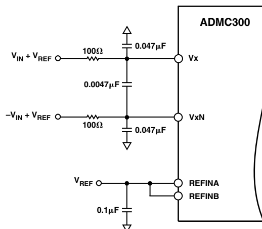
Figure 6. Differential Configuration for ADC Input of ADMC300
