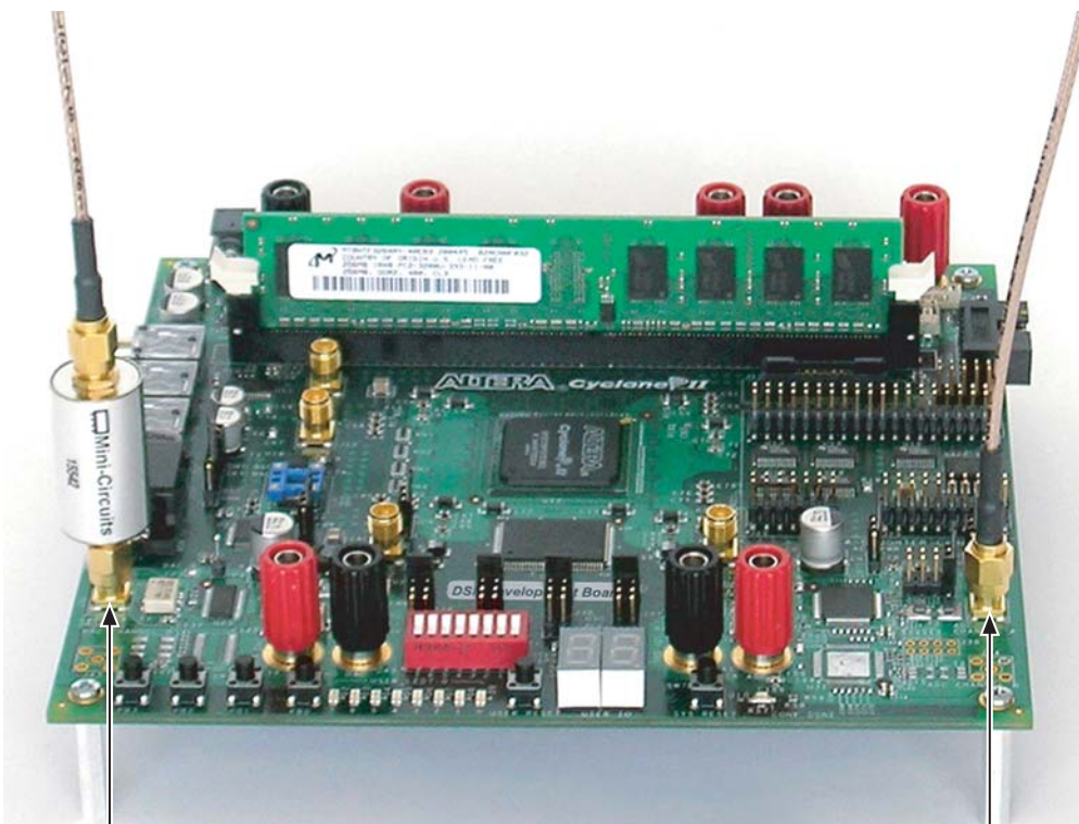
Figure 2-4. SMA Cable & SLP-50 Filter Installed to Connect DAC CHANNEL A (J31) with ADC CHANNEL A (J32)
