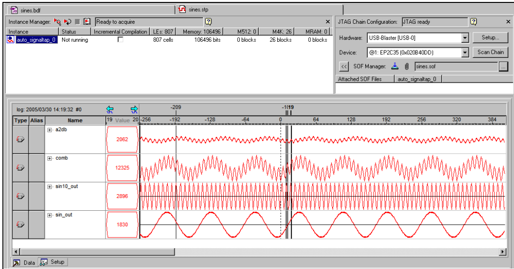
Figure 2–10. Sines.stp Displayed in the SignalTap II Logic Analyzer
