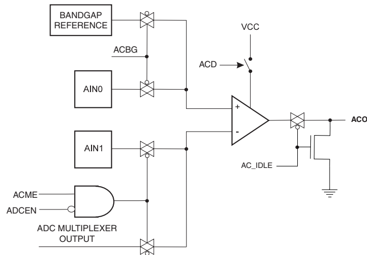
Figure 23-6. Analog Comparator
