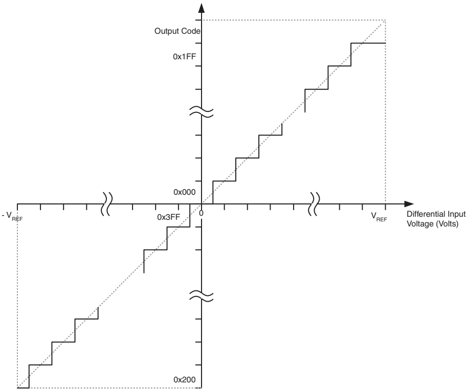
Figure 20-14. Differential Measurement Range
