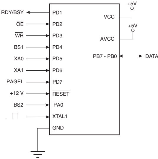
Figure 25-1. Parallel Programming
