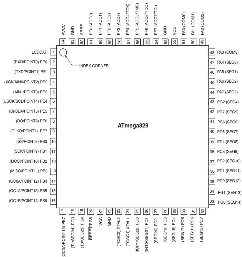
Figure 1-2. Pinout ATmega329P
