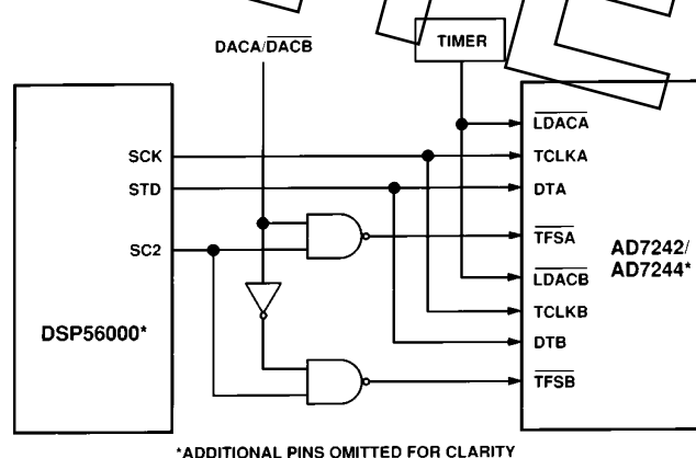
Figure 8. AD7242/AD7244 to DSP56000 Interface
