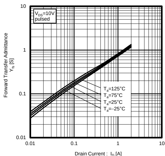
Fig.4 Forward Transfer Admittance vs. Drain Current
