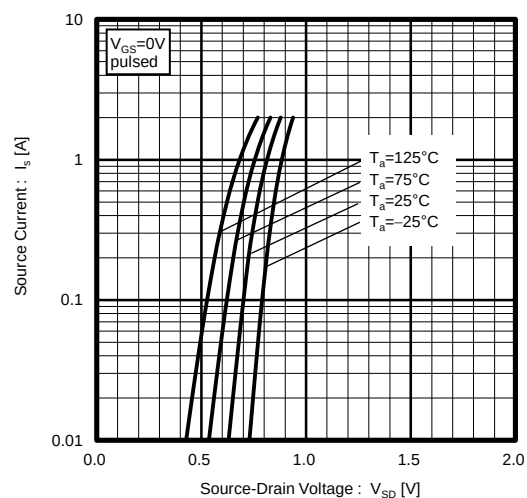
Fig.6 Source Current vs. Source-Drain Voltage
