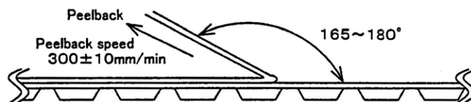
Fig. 8 Test method
