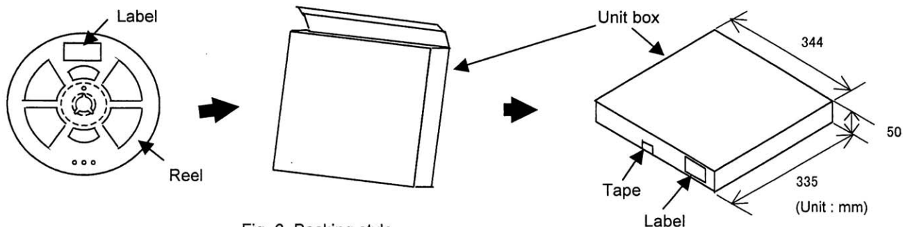
Fig. 6 Packing style
