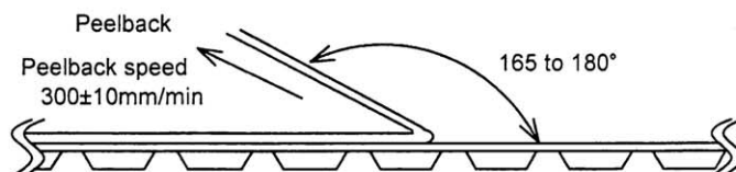
Fig. 8 Test method
