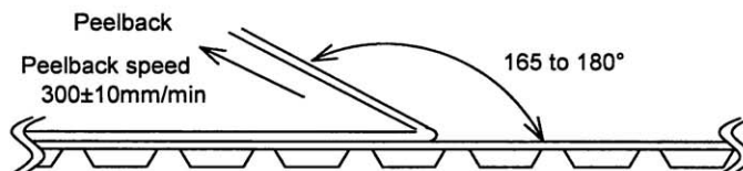
Fig. 8 Test method
