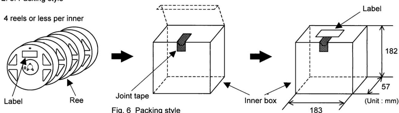
Fig. 6 Packing style
