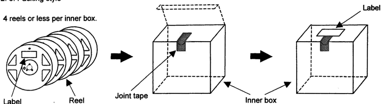
Fig. 6 Packing style
