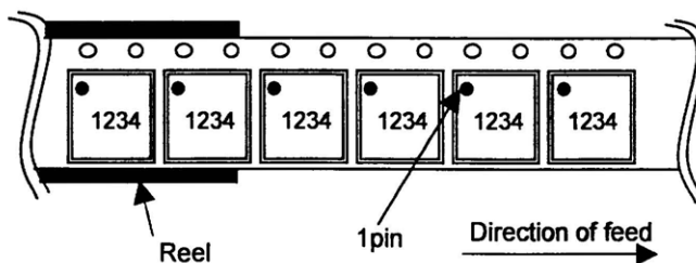
Fig. 2 Typical Tape and Reel configuration
