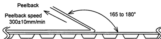
Fig. 8 Test method
