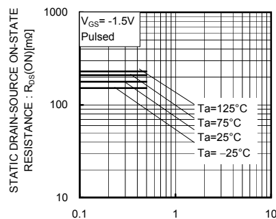
Fig.8 Static Drain-Source On-State Resistance vs. Drain Current( V )
