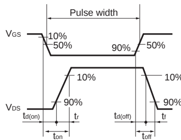
Fig.3-2 Switching waveforms
