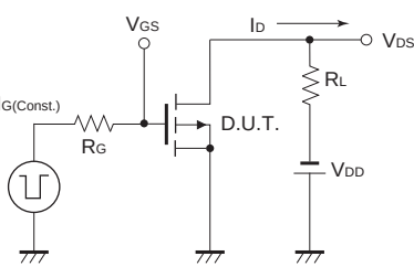
Fig.2-1 Gate Charge Test Circuit
