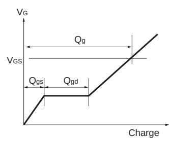
Fig.2-2 Gate Charge Waveform
