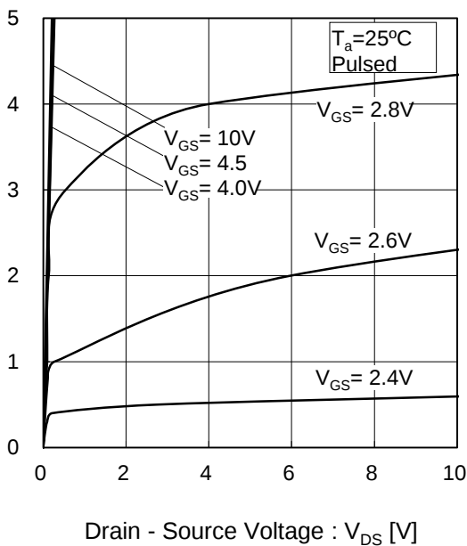
Fig.6 Typical Output Characteristics(II)
