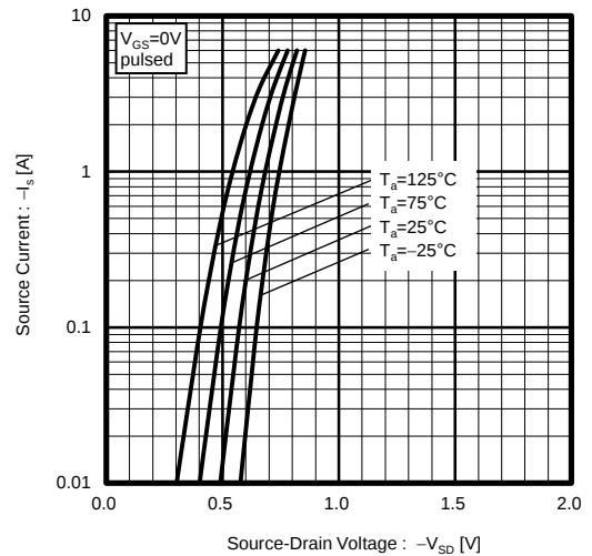
Fig.10 Source Current vs. Source-Drain Voltage
