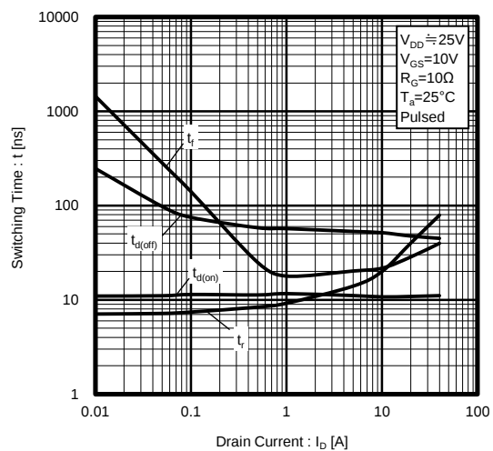
Fig.11 Switching Characteristics
