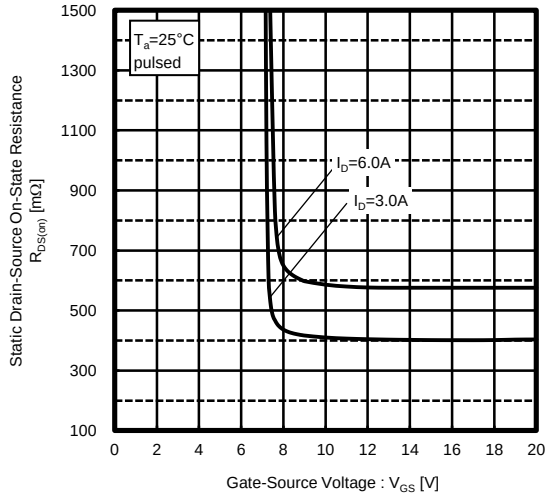
Fig.9 Static Drain-Source On-State Resistance vs. Gate-Source Voltage
